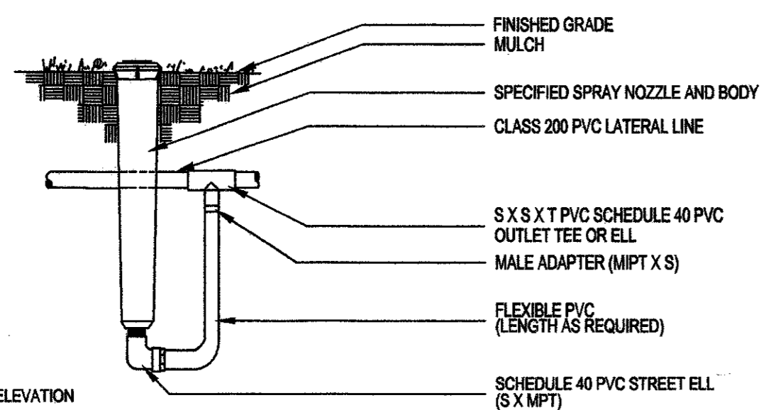
HIGH RISER ASSEMBLY
