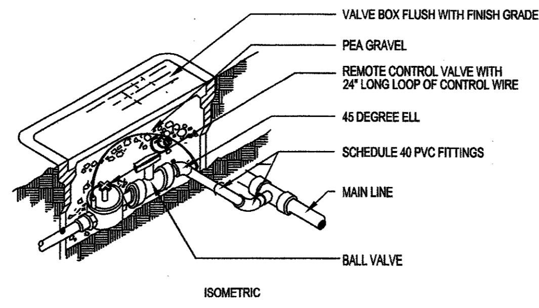
REMOTE CONTROL AND BALL VALVE
