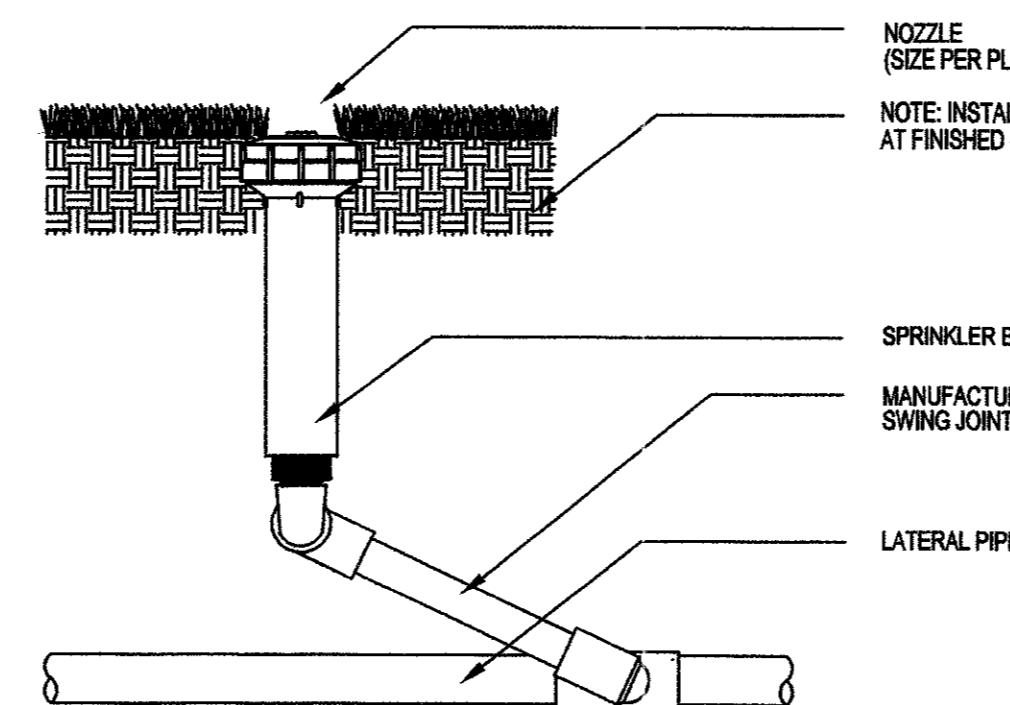
POP - UP RISER ASSEMBLY
