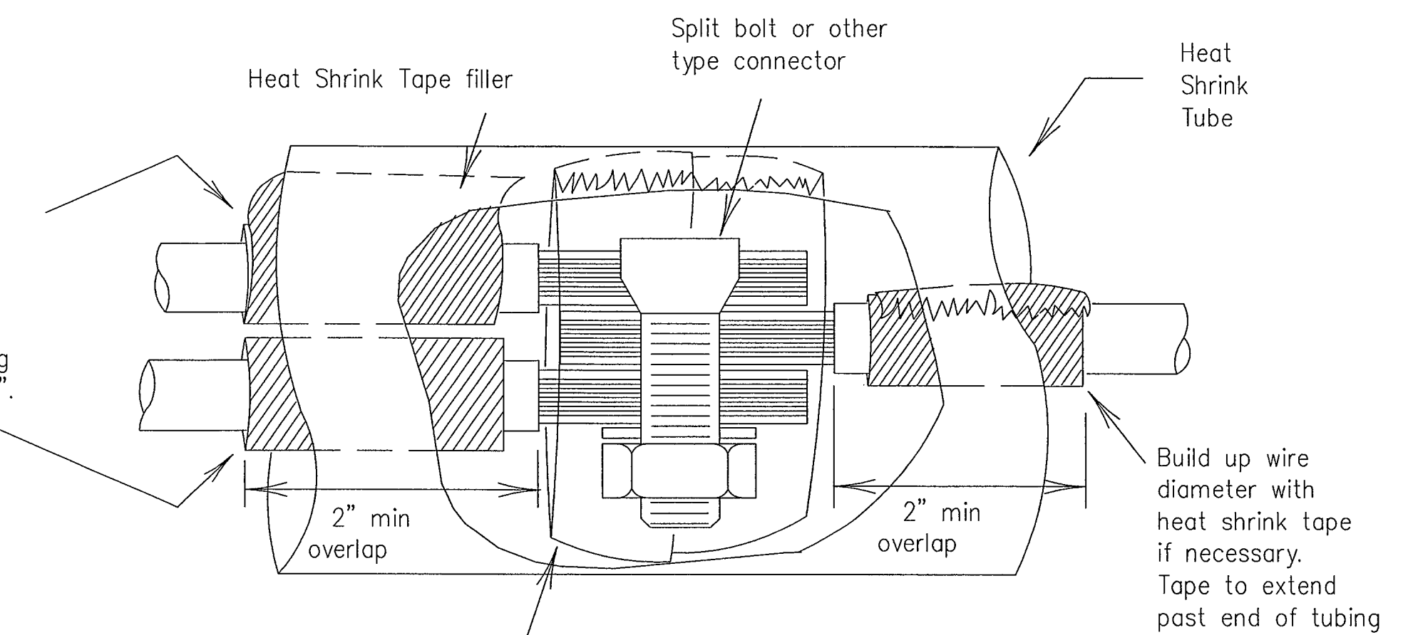
SPLICE OPTION 3 SPLIT BOLT
