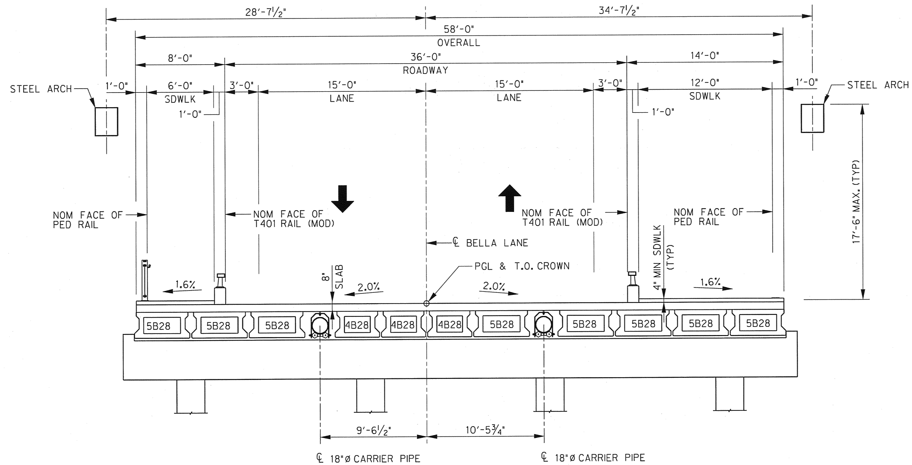
TYPICAL SECTION SCALE: 1" = 10'-0"
