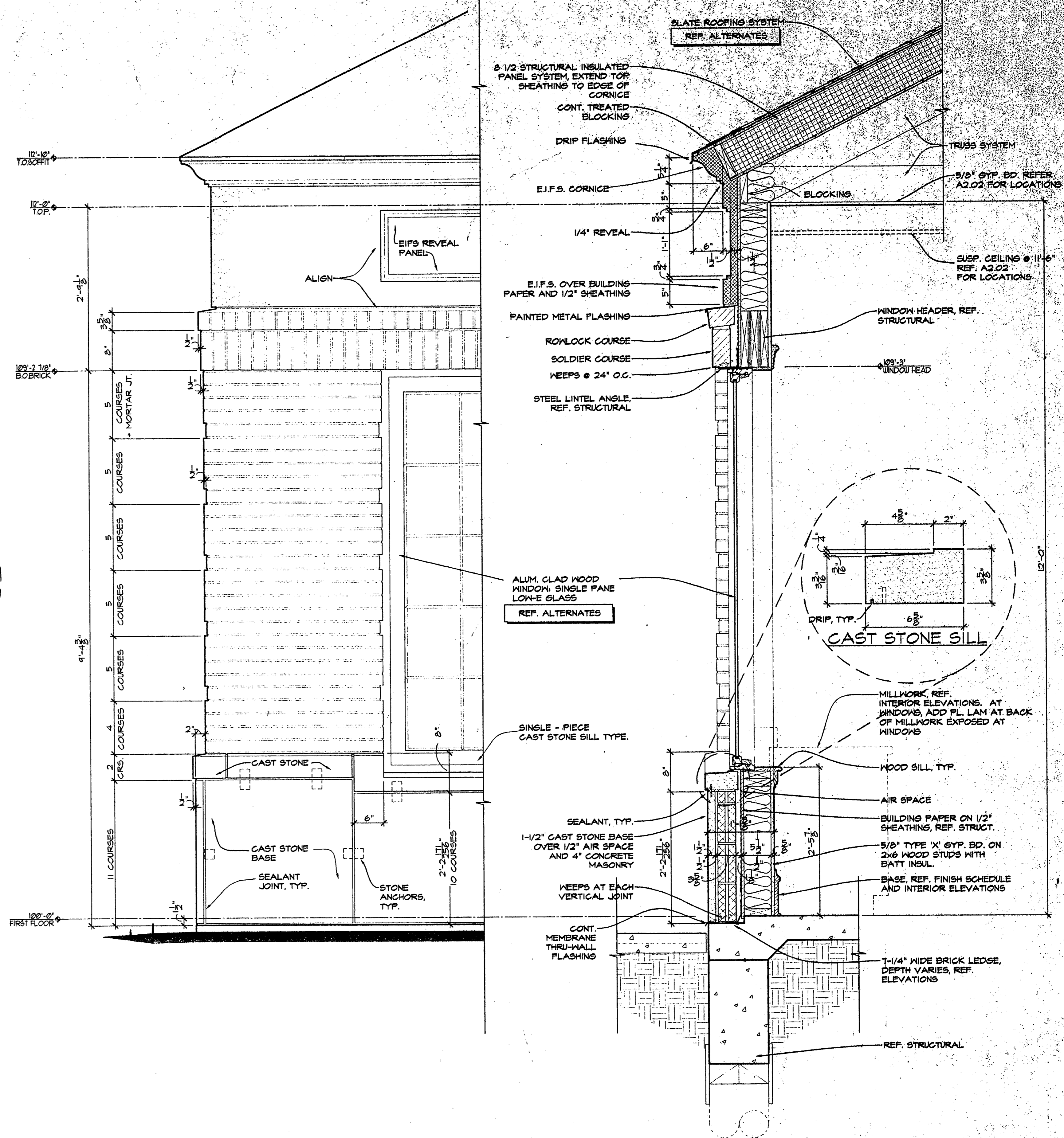
1 WALL SECTION / PARTIAL ELEVATION A4.02 SCALE: 1" = 1'-0"
