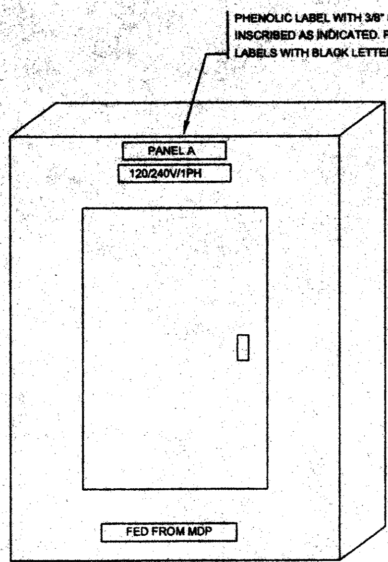
PANELBOARD LABELING DETAIL NO SCALE
