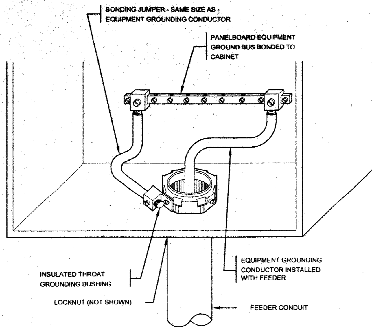
PANELBOARD BONDING DETAIL NO SCALE
