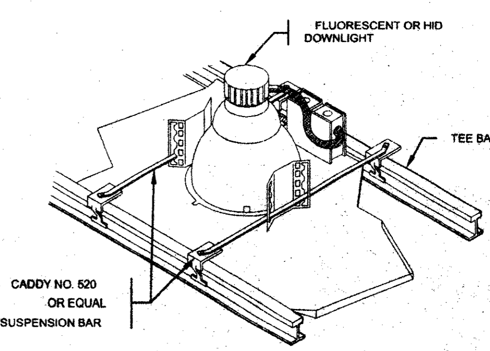
RECESSED CAN LIGHT DETAIL NO SCALE
