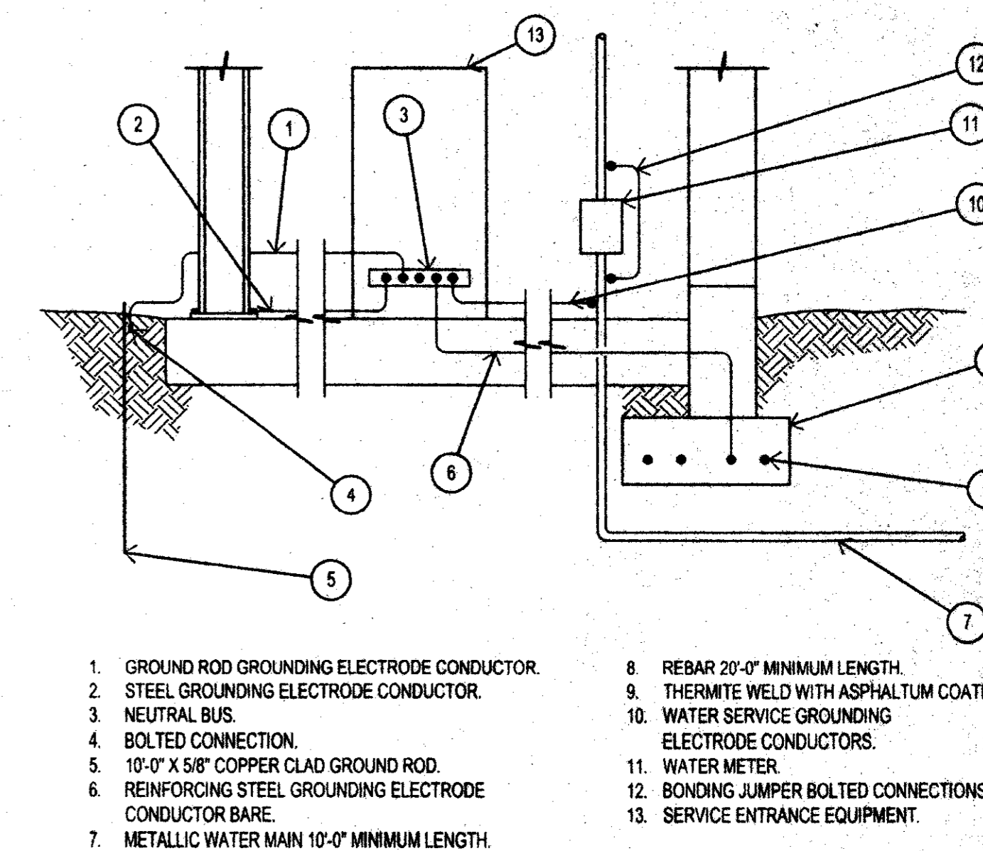
DRIVE-UP UNIT ELECTRICAL DETAIL NO SCALE
