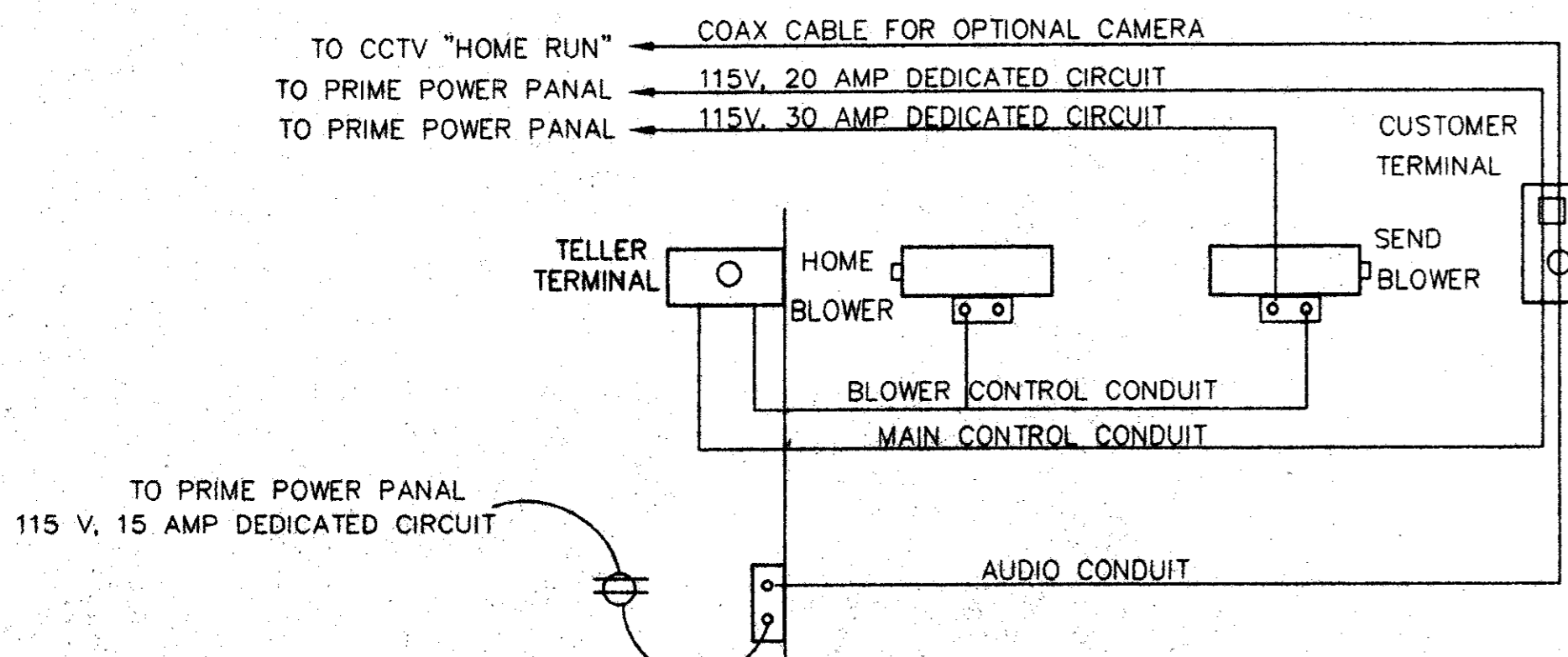
DRIVE-UP UNIT BLOCK DIAGRAM NO SCALE
