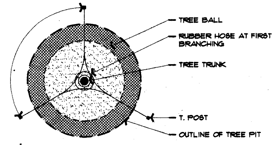
Tree Planting Plan NTS
