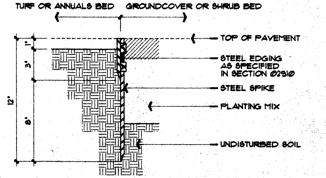
Steel Edging Section NTS
