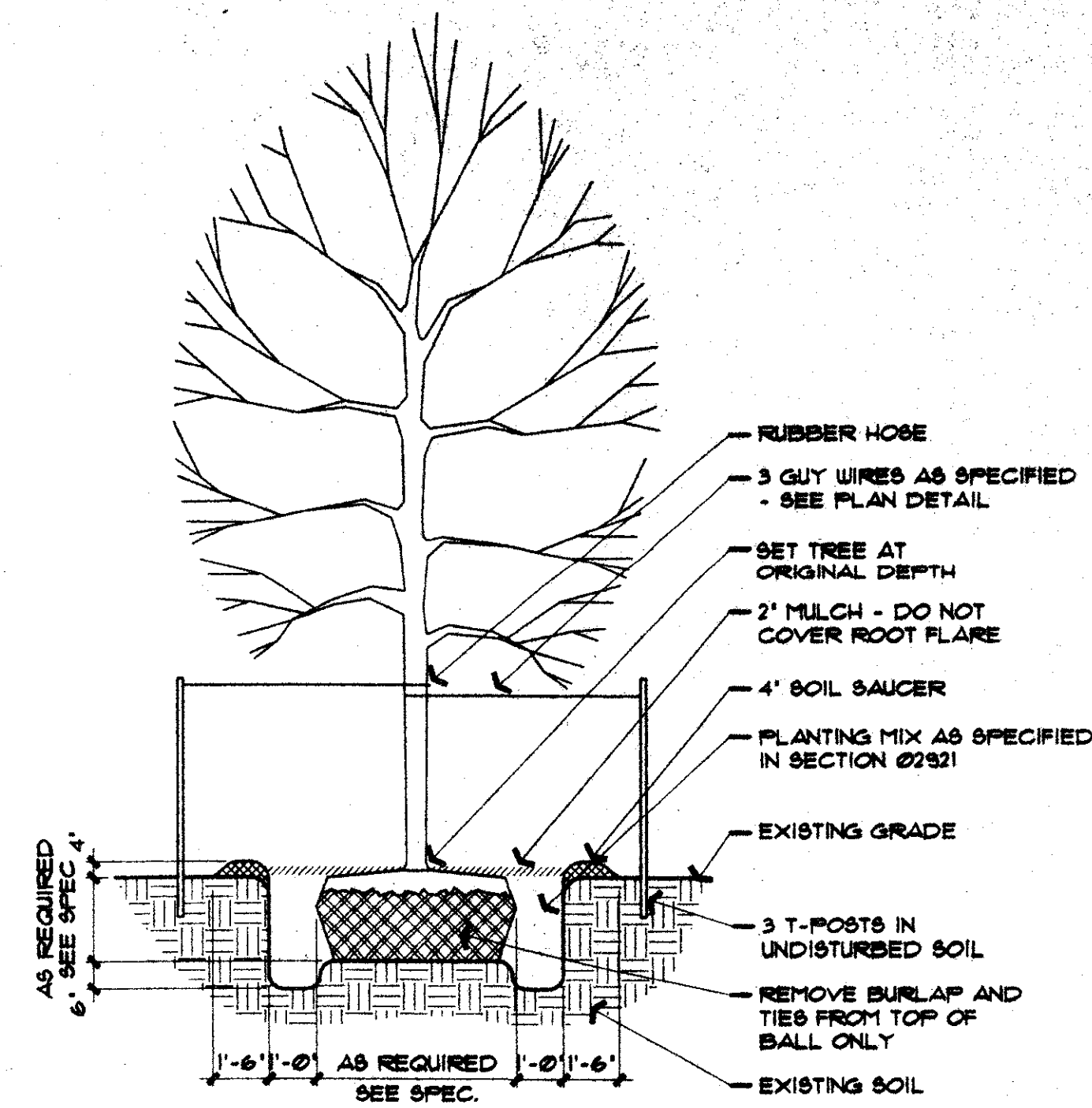
Tree Planting Section NTS
