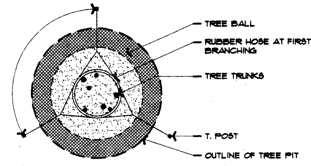
Ornamental Tree Planting Plan NTS
