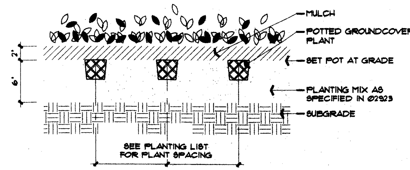
Groundcover Planting Section NTS
