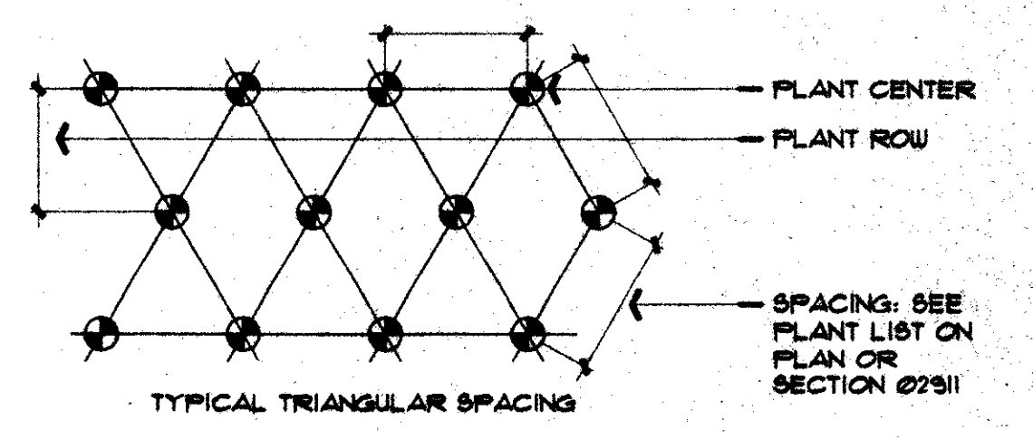
Plant Spacing Plan NTS
