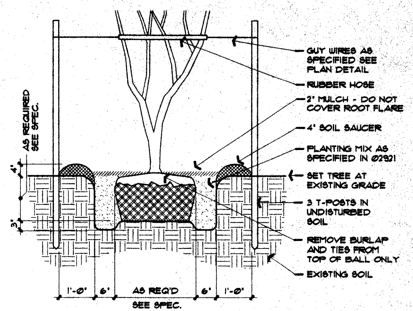
Ornamental Tree Planting Section NTS
