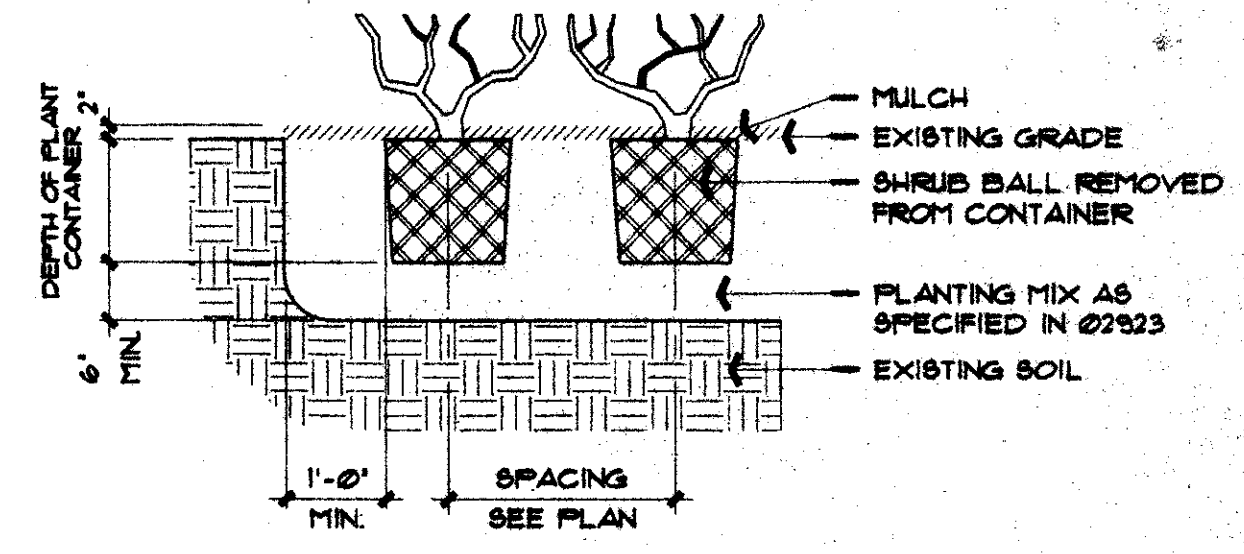
Shrub Planting Section NTS
