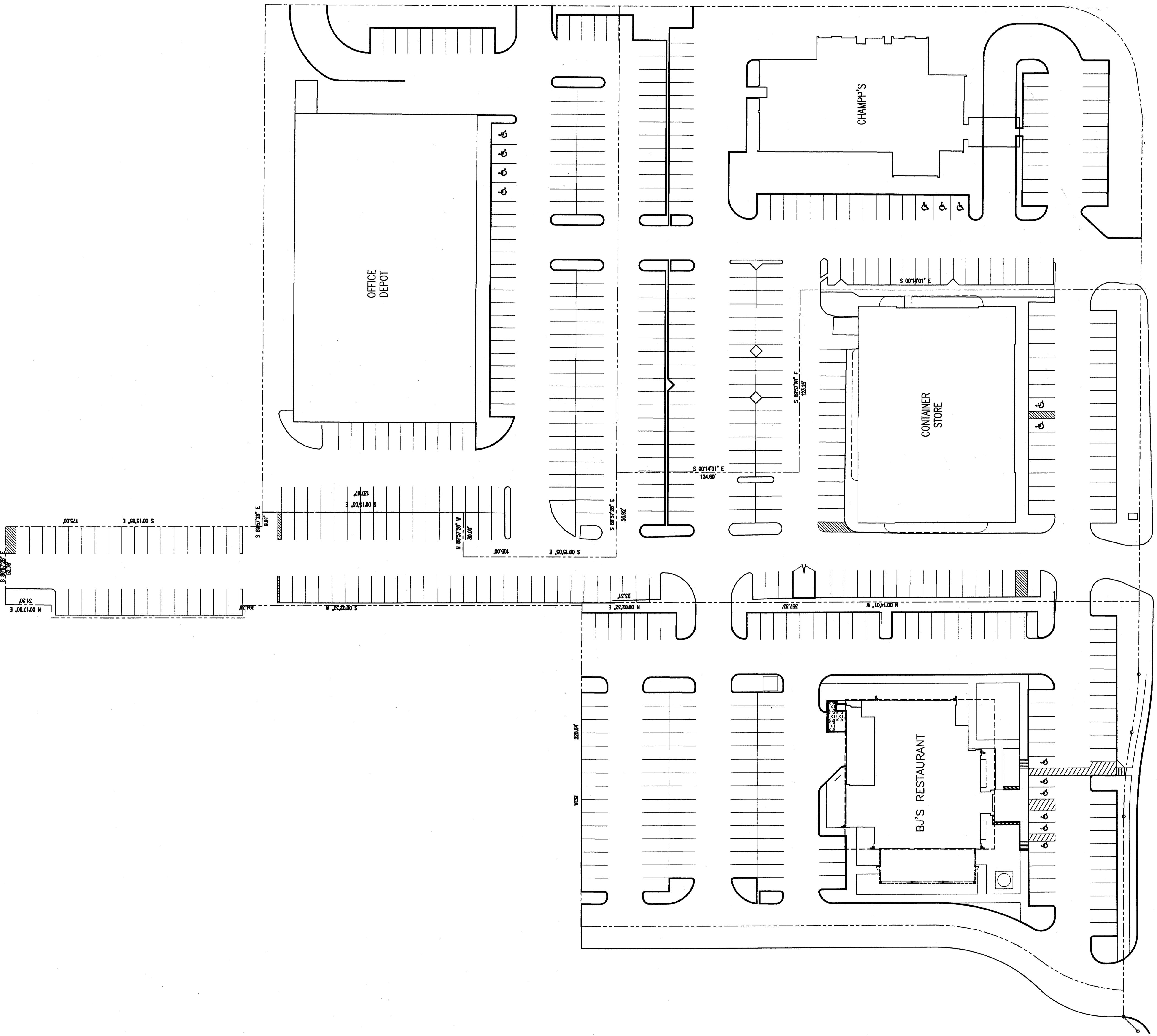
01 EXISTING SITE PLAN SCALE: 1" = 30'-0" X-EXIST. SITE020
