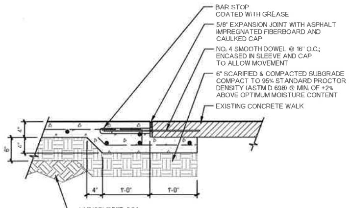
07 NEW TO OLD CONCRETE CONNECTION SCALE: 1" = 1'-0" SECTION
