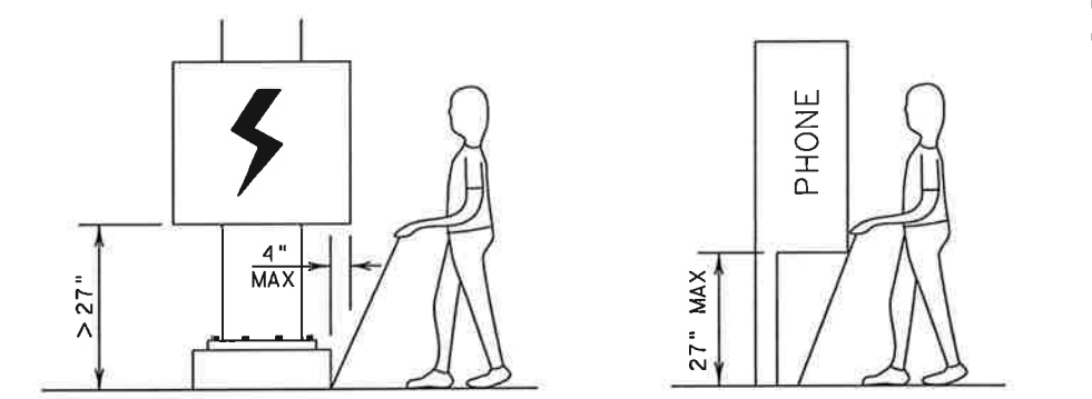
When an obstruction of a height greater than 27" from the surface would create a protrusion of more than 4" into the pedestrian circulation area, construct additional curb or foundation at the bottom to provide a maximum 4" overhang. Protruding objects of a height ≤ 27" are detectable by cane and do not require additional treatment.
