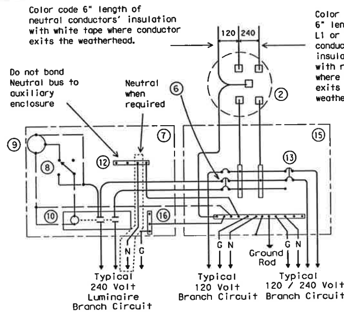
SCHMATIC TYPE I 120/240 VOLTS - THREE WIRE
