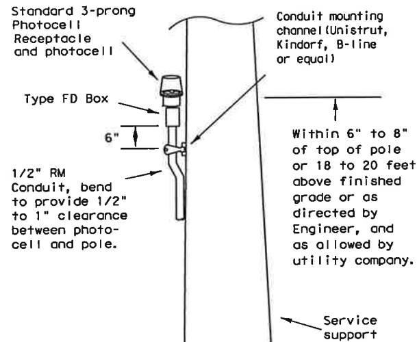
TOP MOUNTED PHOTOCELL
