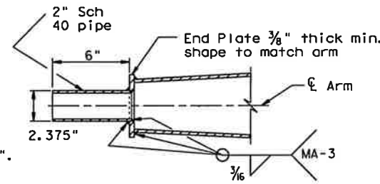
TENON DETAIL
