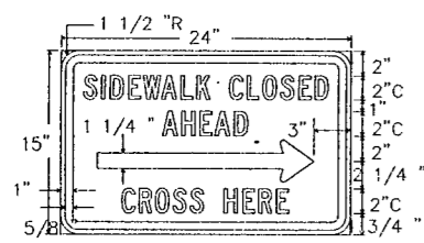
R5-9a 24" X 15" Letters - Black Symbol - Black Border - Black Background - White Refl.
