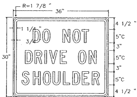
R4-3a 36" X 30" Letters - Black Border - Black Background - White Refl.
