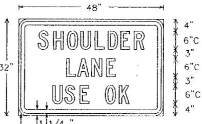
R4-3d 48" X 32" Letters - Black Border - Black Background - White Refl.
