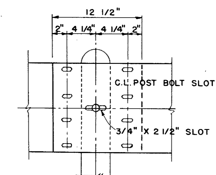
RAIL SPLICE
