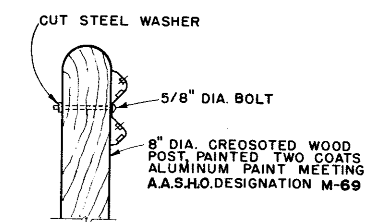
ARRANGEMENT AT POSTS
