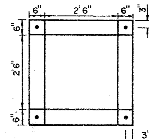
Sect. "C-C"
