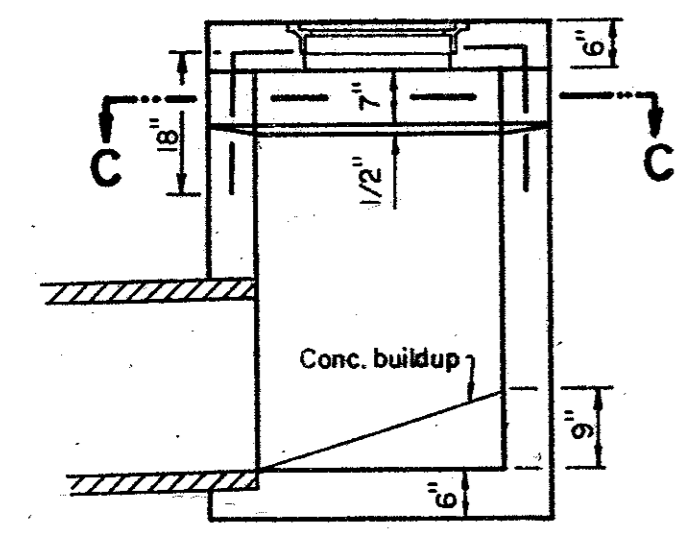
Sect. "A-A"
