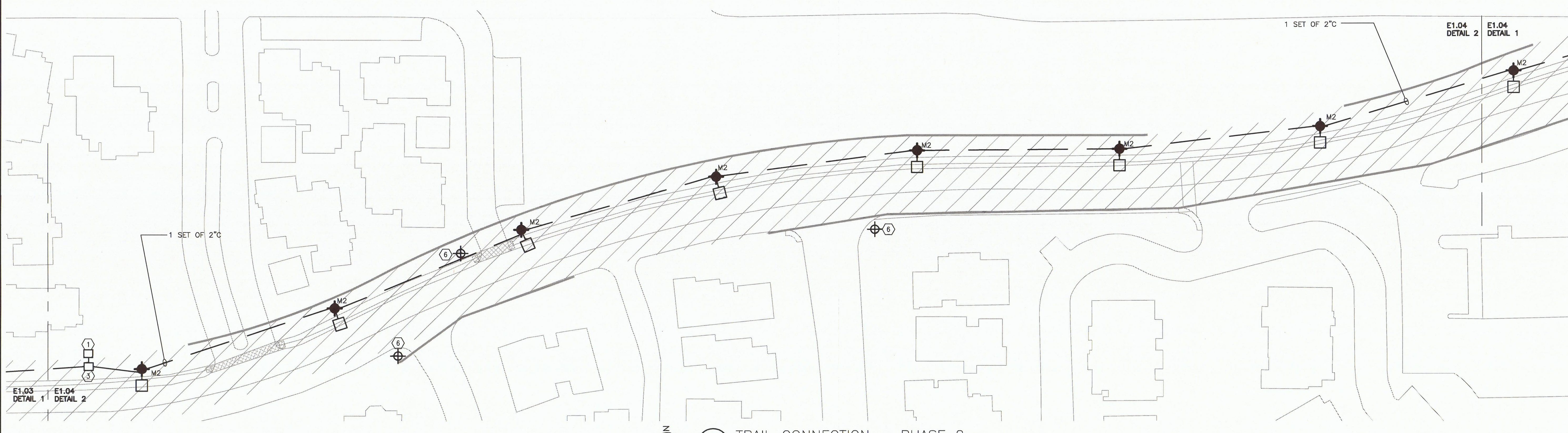
2 TRAIL CONNECTION - PHASE 2 SCALE: 1" = 40'-0"
