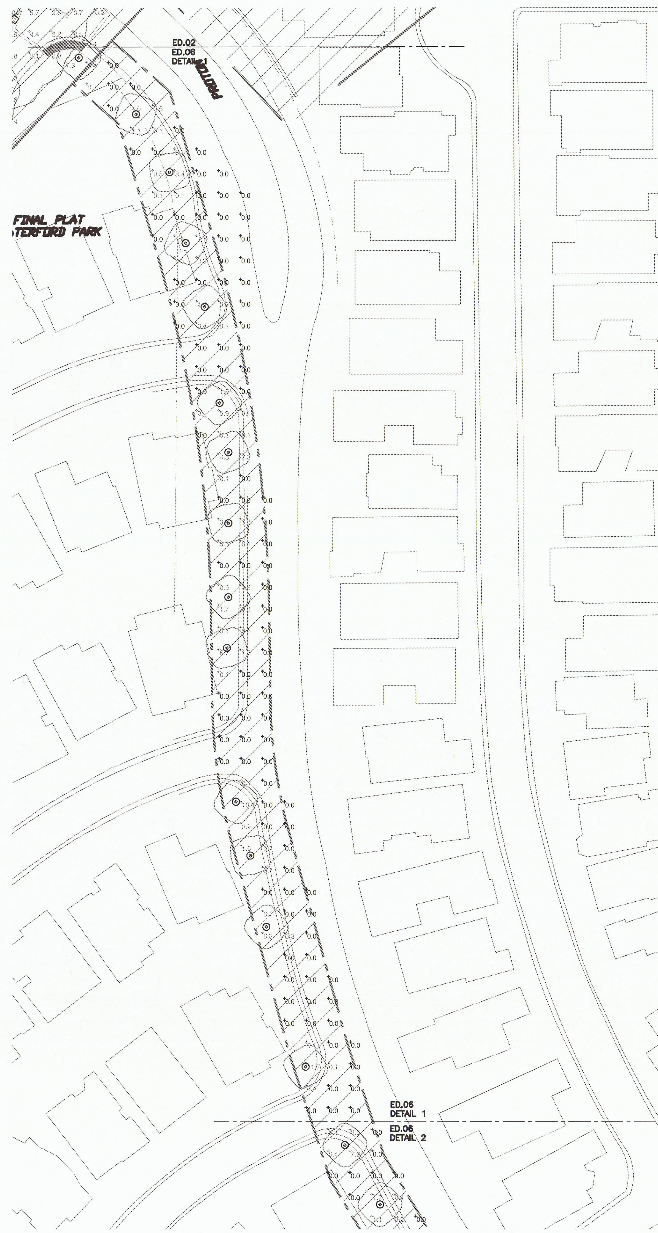
1 TRAIL CONNECTION - PHASE 3 SCALE: 1" = 40'-0"
