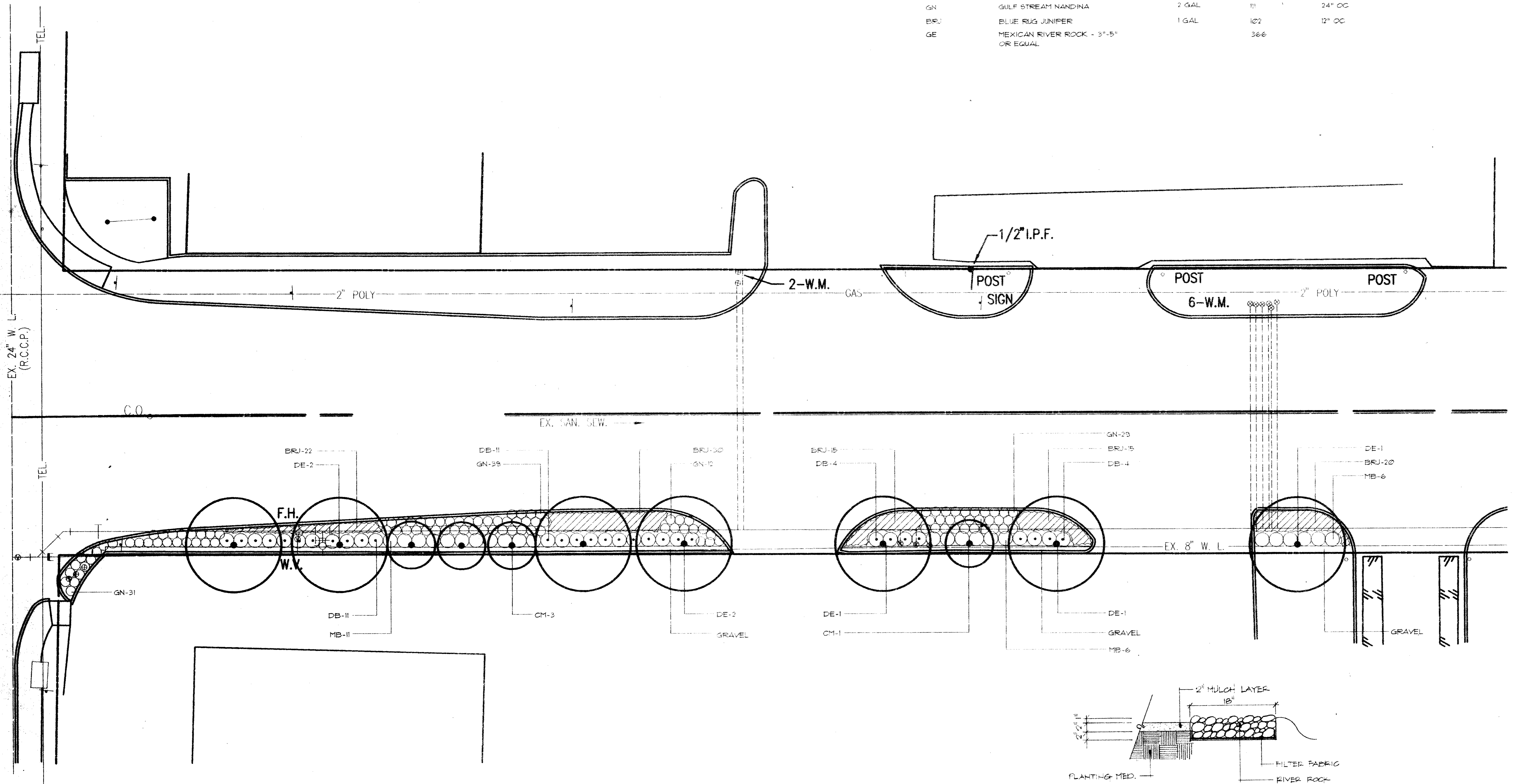
ROCK EDGING DETAIL 1'-1'-0"
