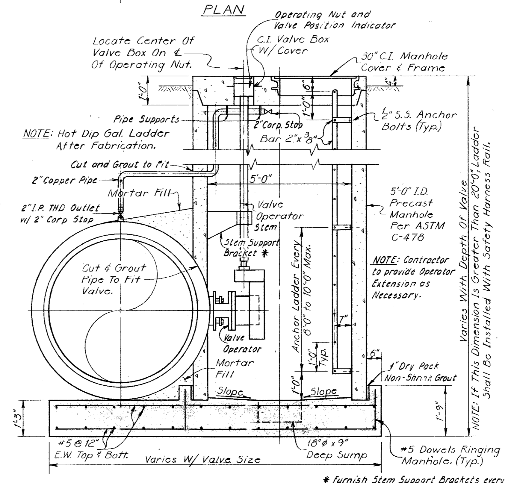
TYPICAL BUTTERFLY VALVE INSTALLATION 1/2"=1'-0"
