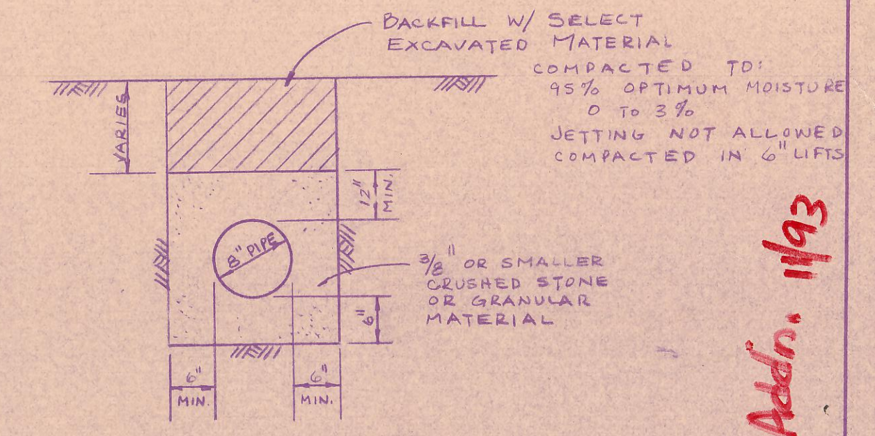
EMBEDMENT DETAIL - SANITARY SEWER N.T.S.
