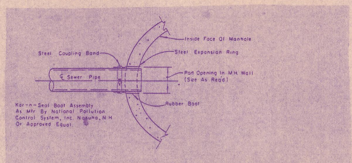
TYPICAL SEWER CONNECTION AT MANHOLE
