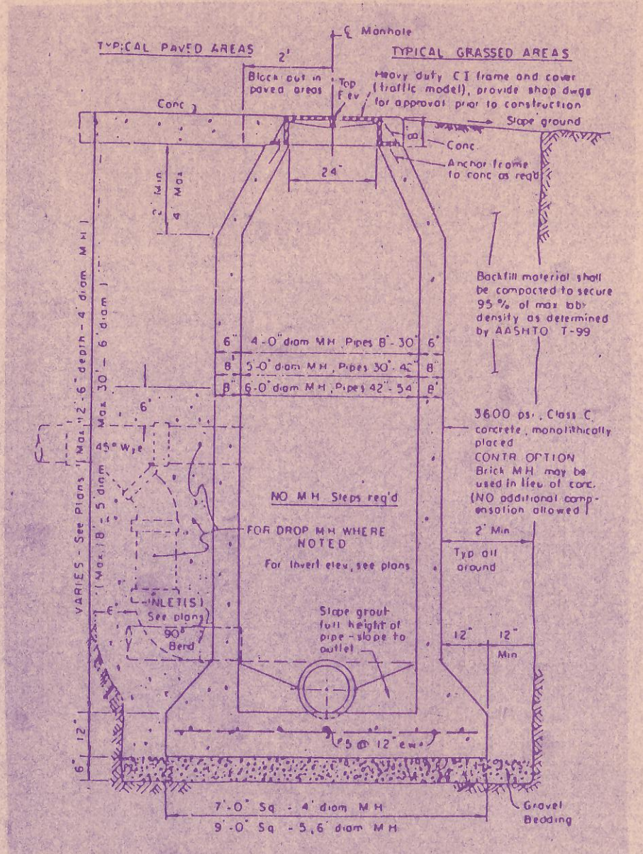
CAST IN PLACE MANHOLE WHERE DROP MH IS REQUIRED, USE INSIDE DROP CONNECTION AS PER TOWN OF ADDISON STANDARDS.
