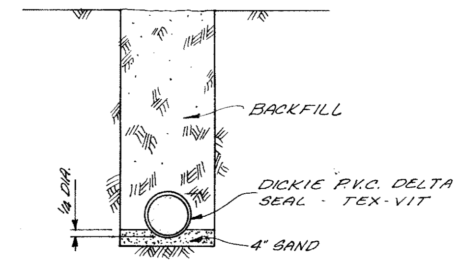
CLASS A EMBEDMENT SCALE 2" = 1'-0"
