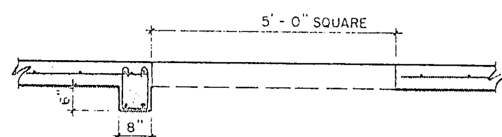
SECTION 3 SCALE - 1/2" = 1'-0"
