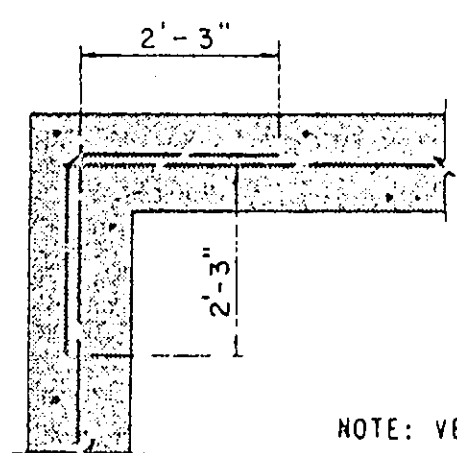
TYPICAL CORNER REINFORCING DETAILS (PLAN VIEW)
