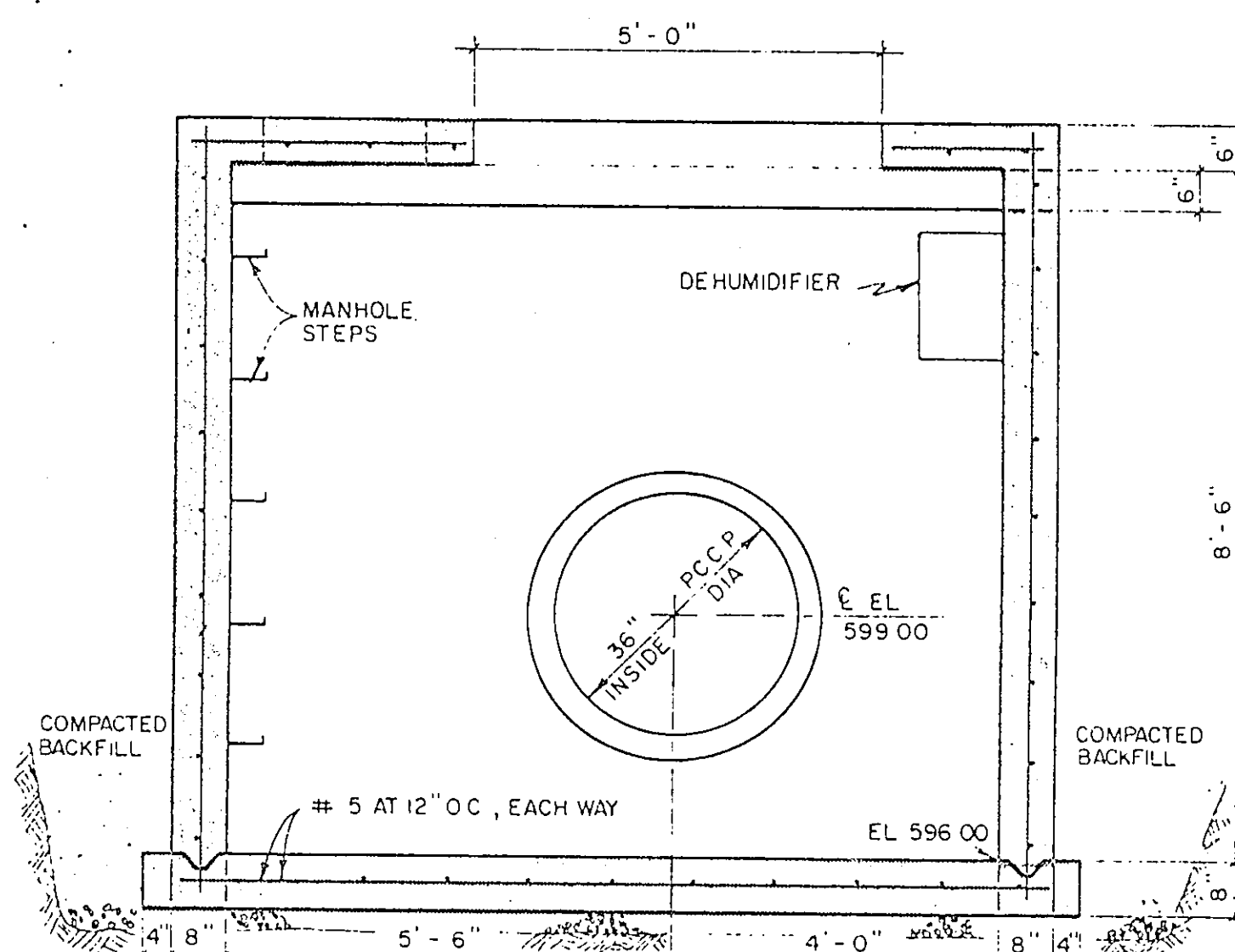
SECTION 2 SCALE - 1/2" = 1'-0"
