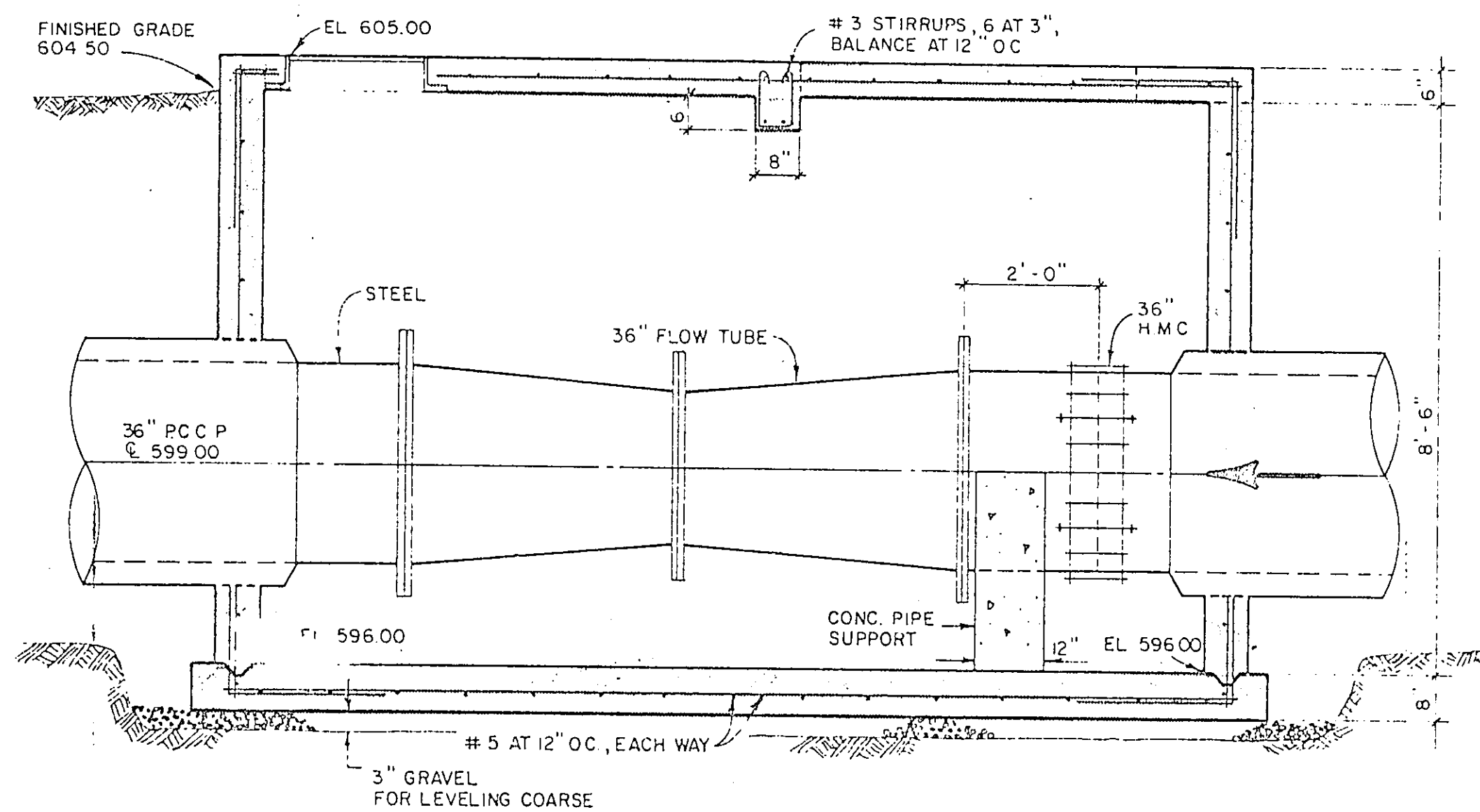
SECTION 1 SCALE - 1/2" = 1'-0"
