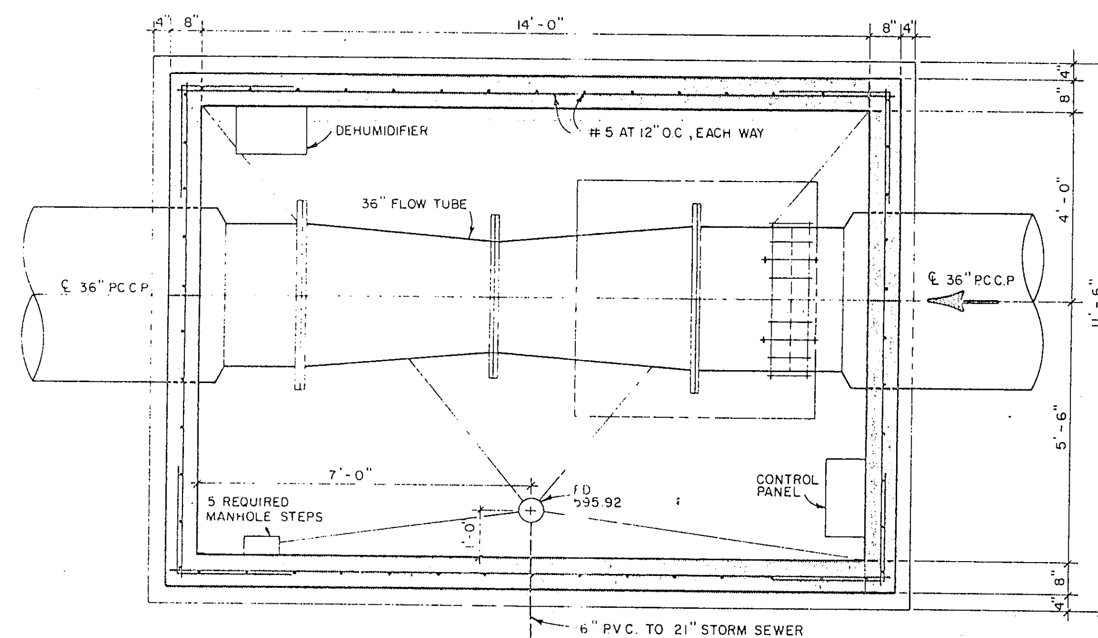
SECTIONAL PLAN SCALE - 1/2" = 1'-0"
