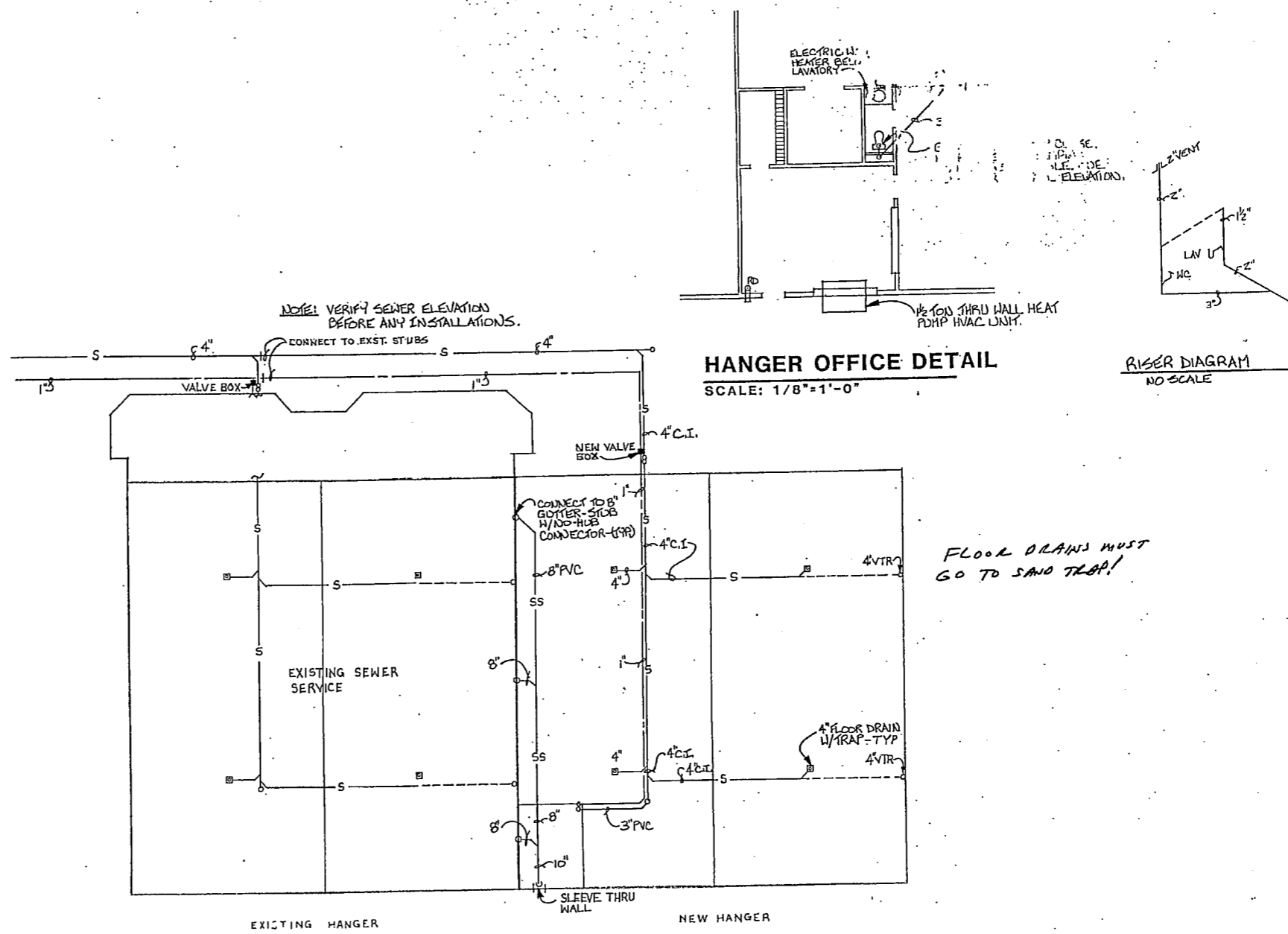
PLAN VIEW - PLUMBING LAYOUT SCALE: 1"=20'-0"
