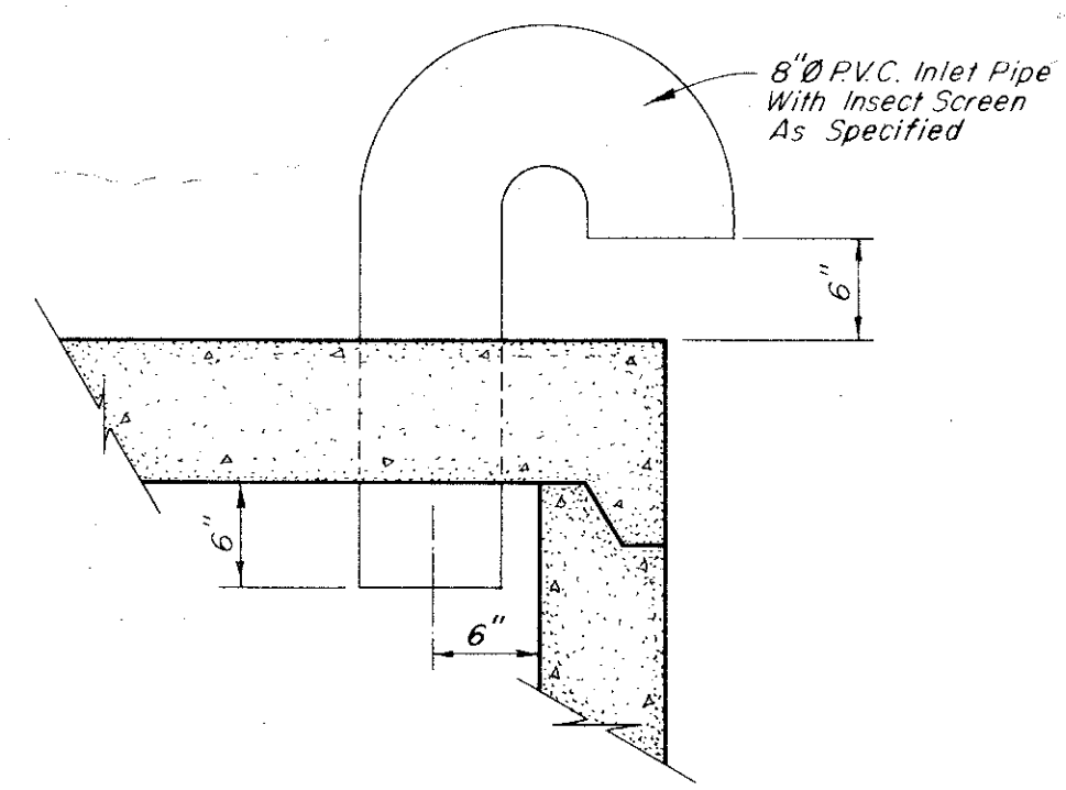
INLET PIPE DETAIL No Scale
