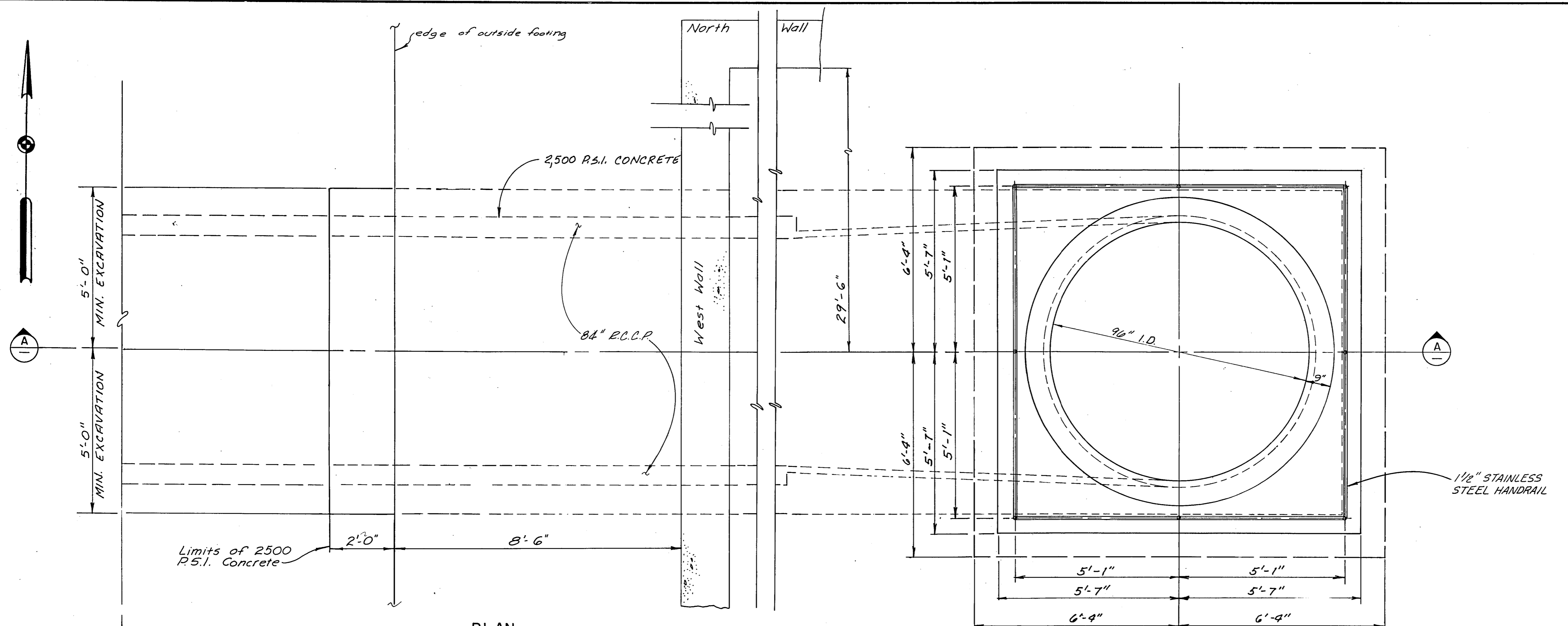
PLAN RESERVOIR INLET SCALE: 1/2" = 1'-0"
