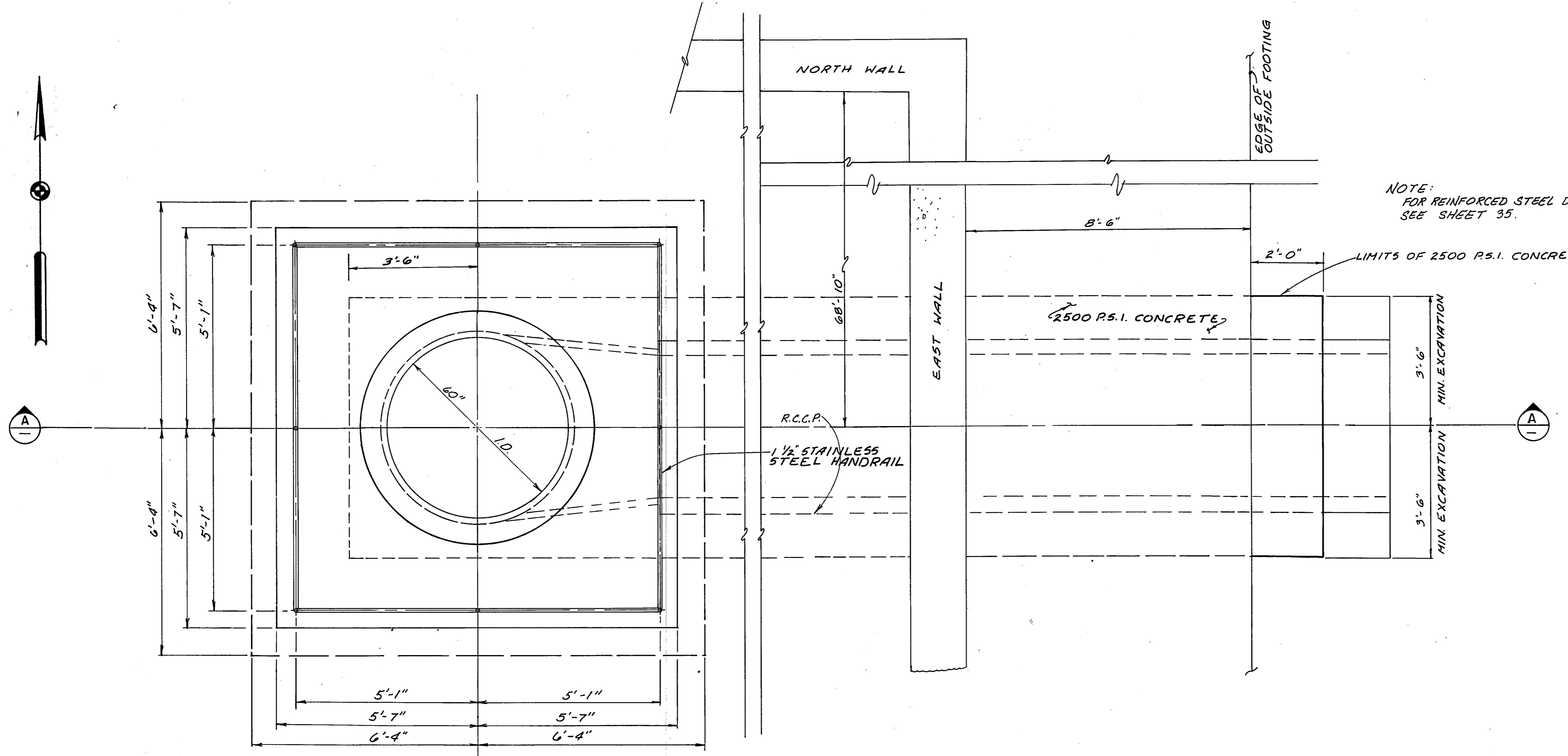
PLAN RESERVOIR OUTLET SCALE: 1/2" = 1'-0"
