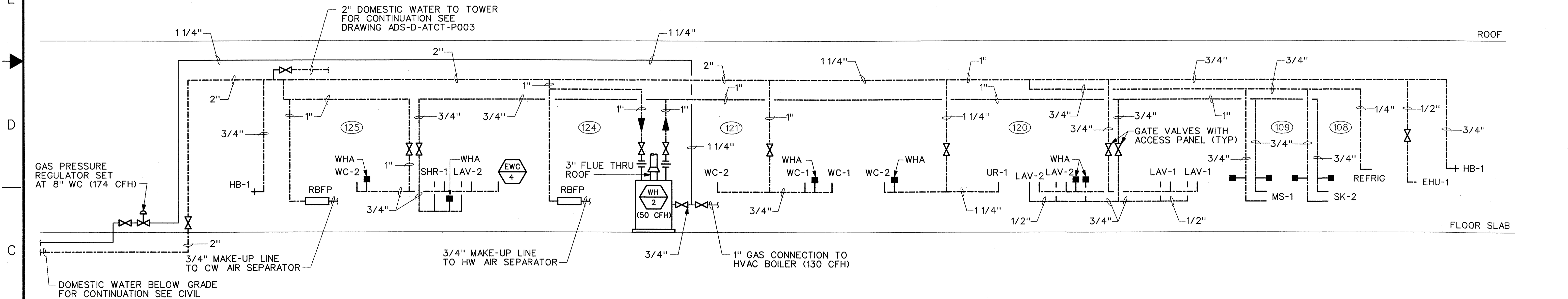
DOMESTIC WATER AND NATURAL GAS RISER DIAGRAM - BASE - EG BUILDING
