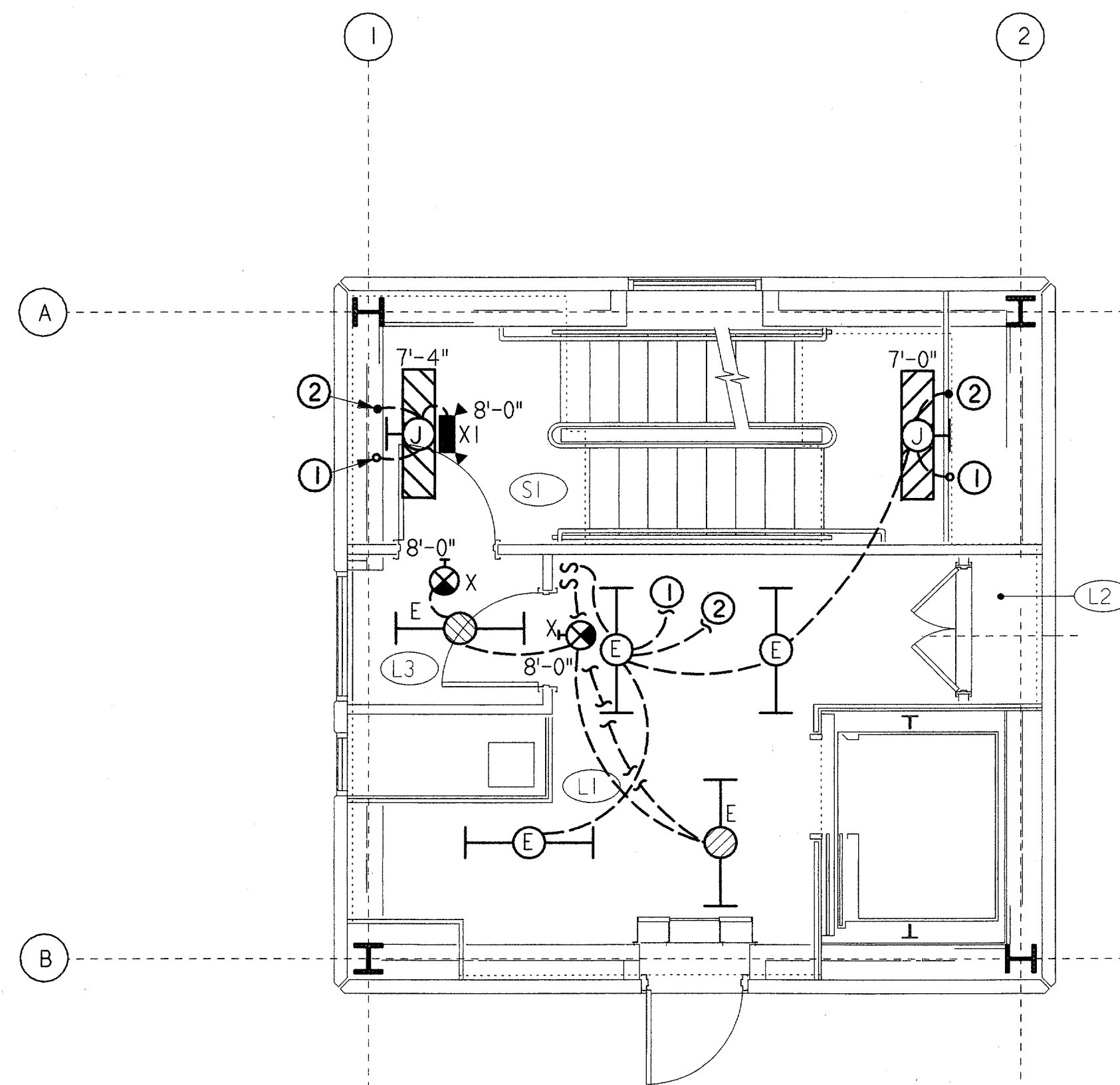
JUNCTION LEVEL 1/4" = 1'-0" EL = 40'-0"
