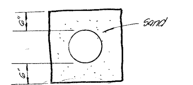
TYPICAL EMBEDMENT FOR WATER & SANITARY SEWER No Scale
