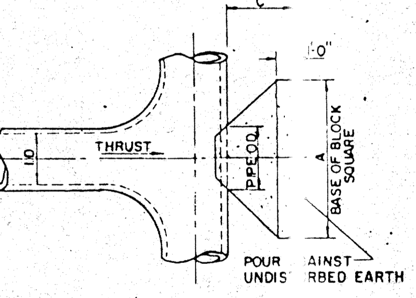
PLAN OF TEE THRUST BLOCK
