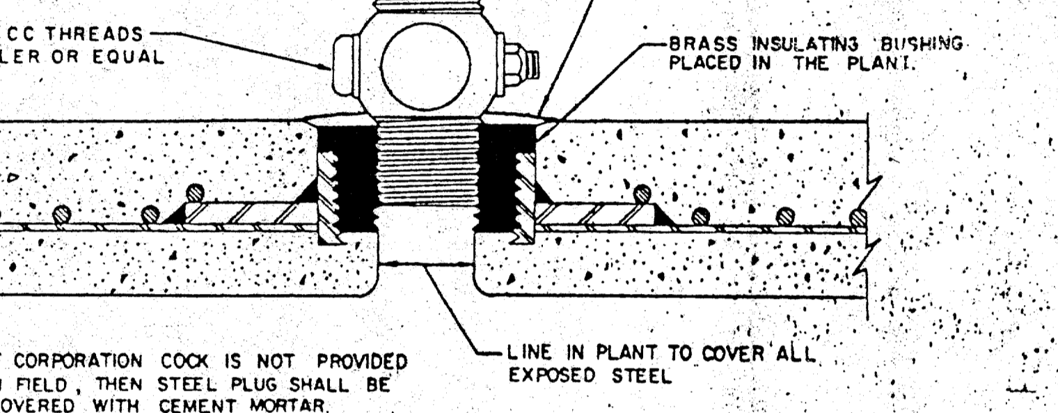
THREADED CONNECTION
