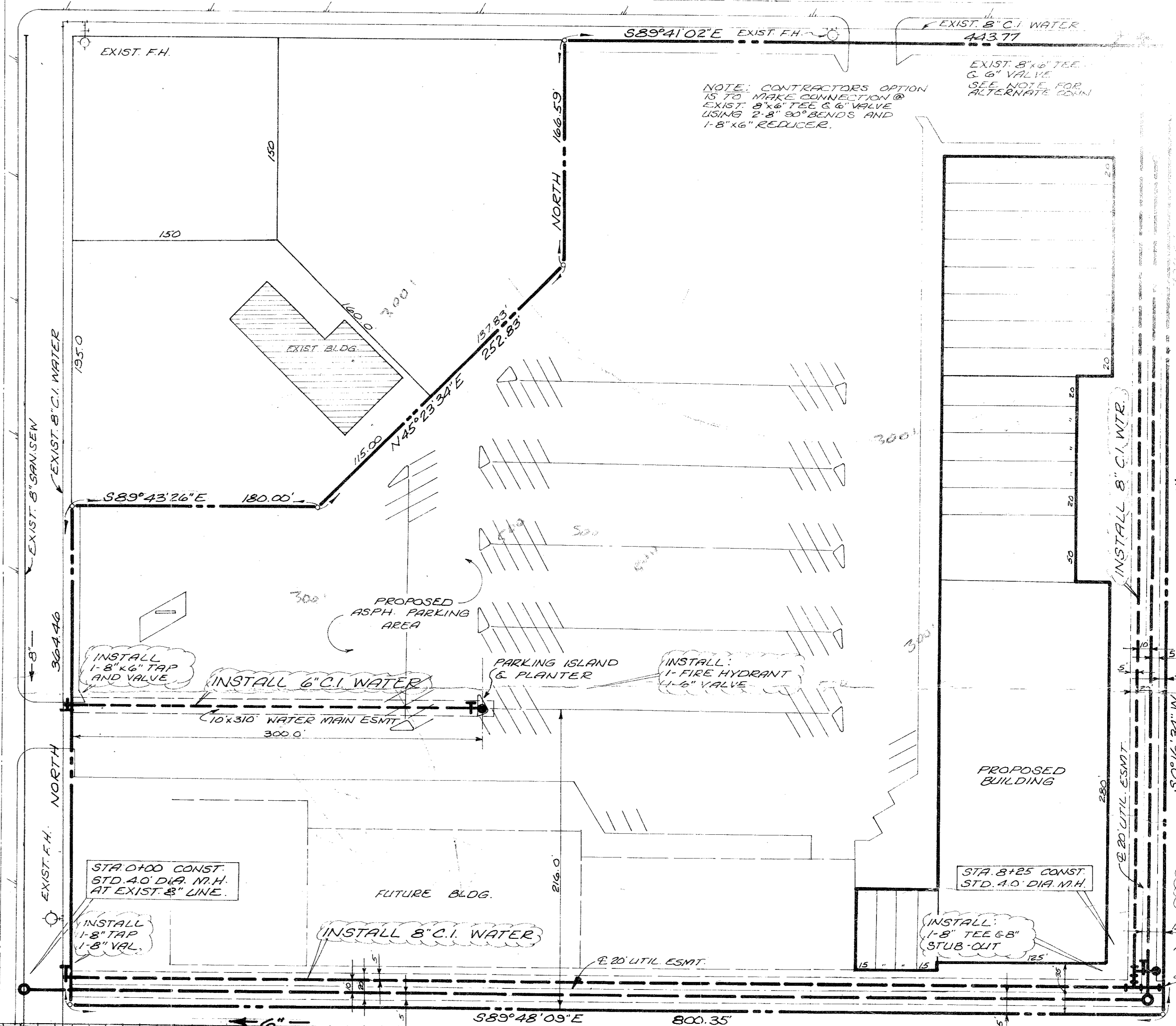
PLAN SCALE 1"=50'
