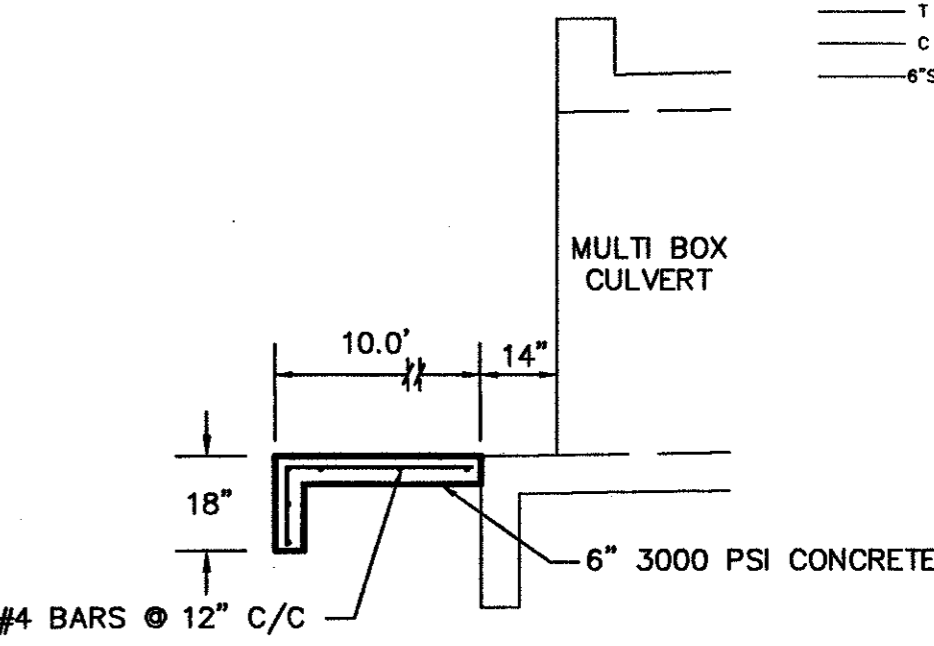
Channel Lining Section "C-C" NOT TO SCALE
