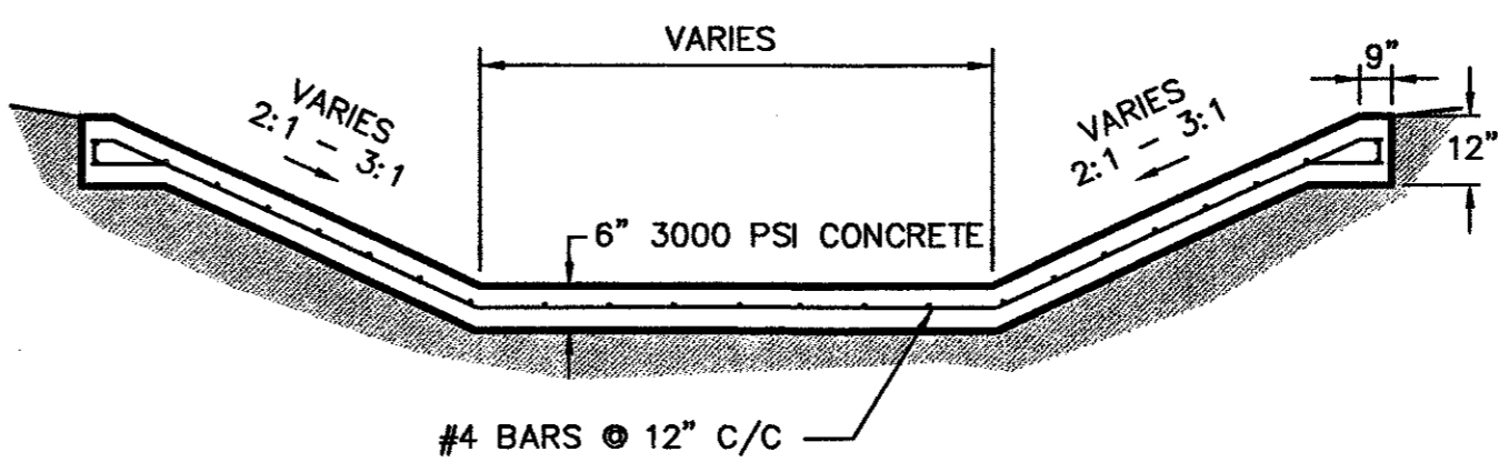
Channel Lining Section "B-B" NOT TO SCALE
