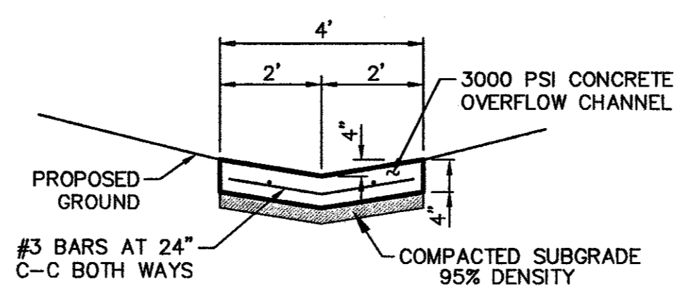
VIEW "A-A" NOT TO SCALE
