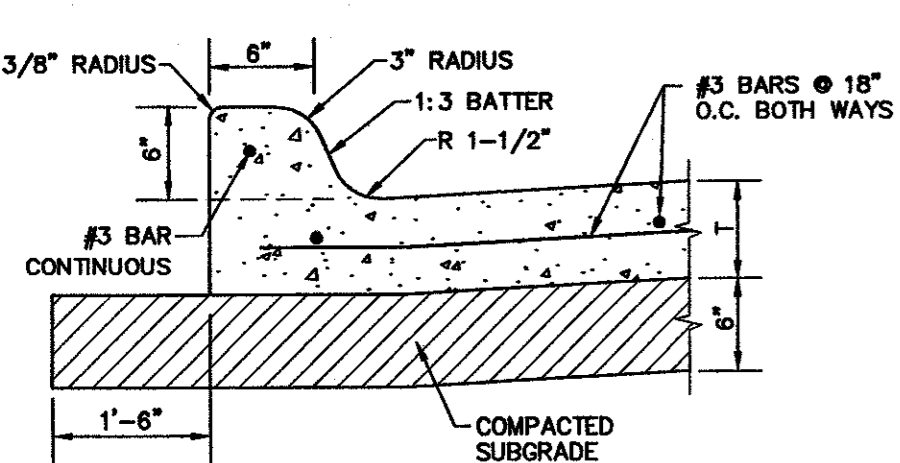
1 INTEGRAL CURB NOT TO SCALE
