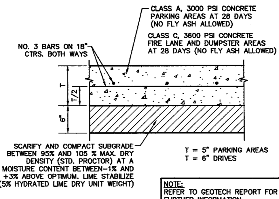
2 CONCRETE PAVEMENT SECTION NOT TO SCALE
