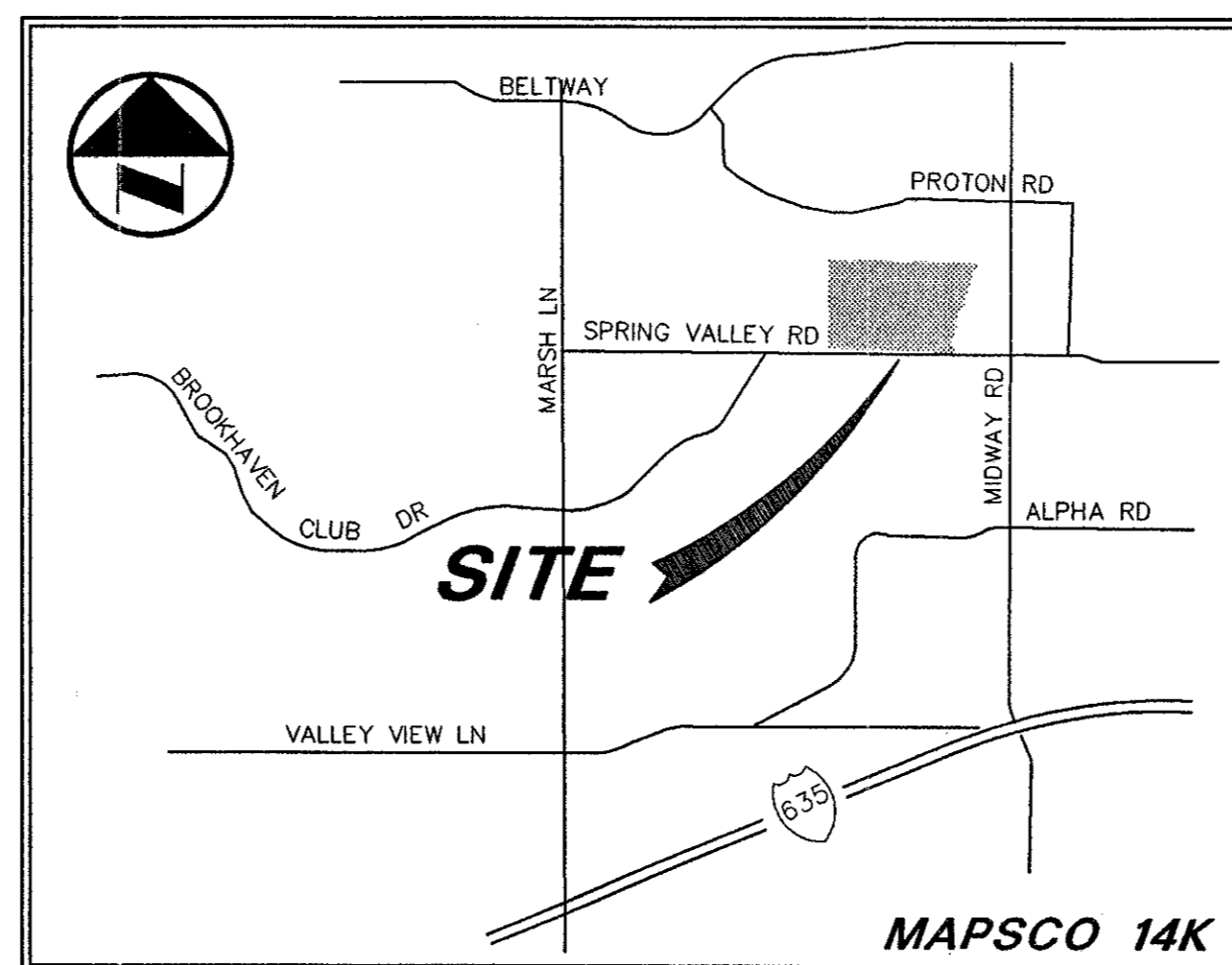
VICINITY MAP
