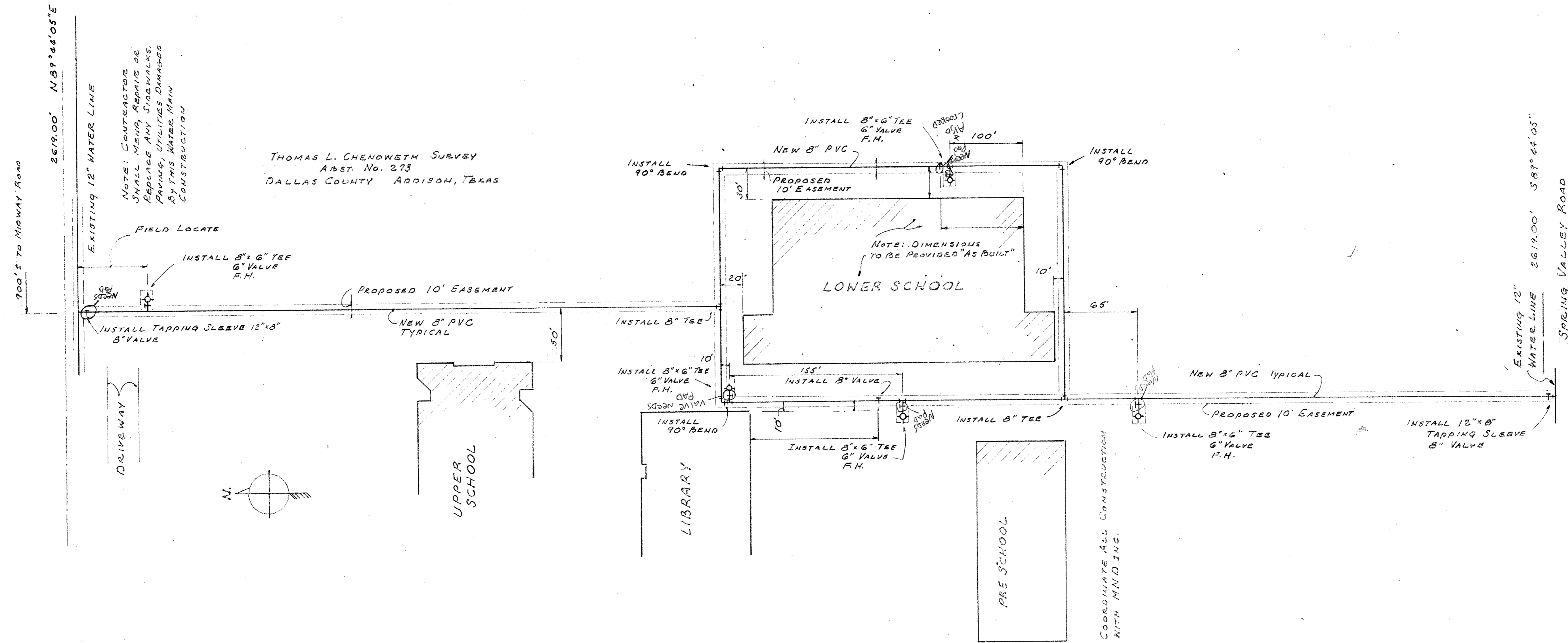
PROPOSED WATER DISTRIBUTION PLAN 1" = 50'
