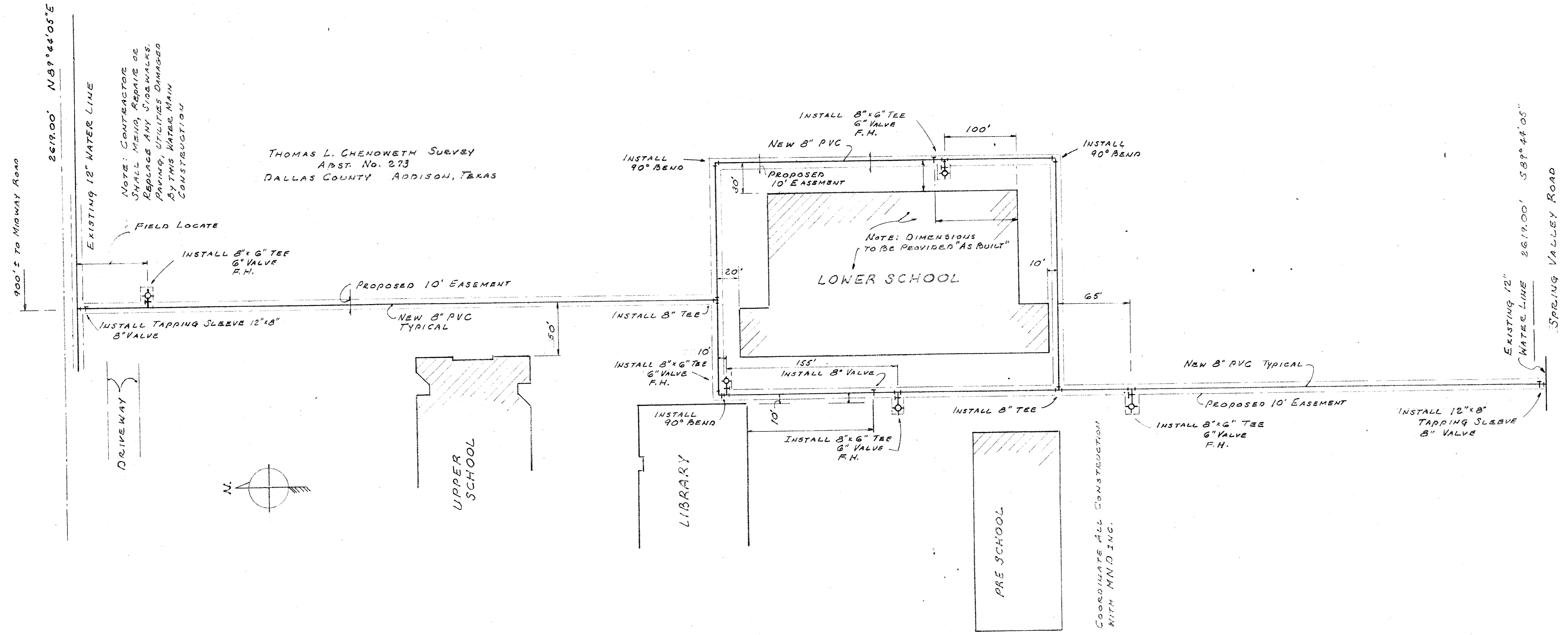
PROPOSED WATER DISTRIBUTION PLAN 1" = 50'
