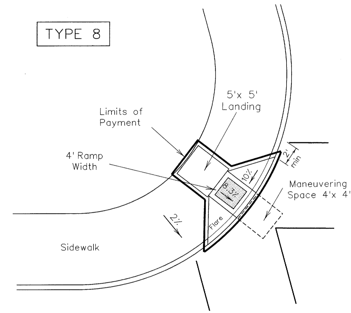
DIAGONAL CURB RAMP (FLARED SIDES)
