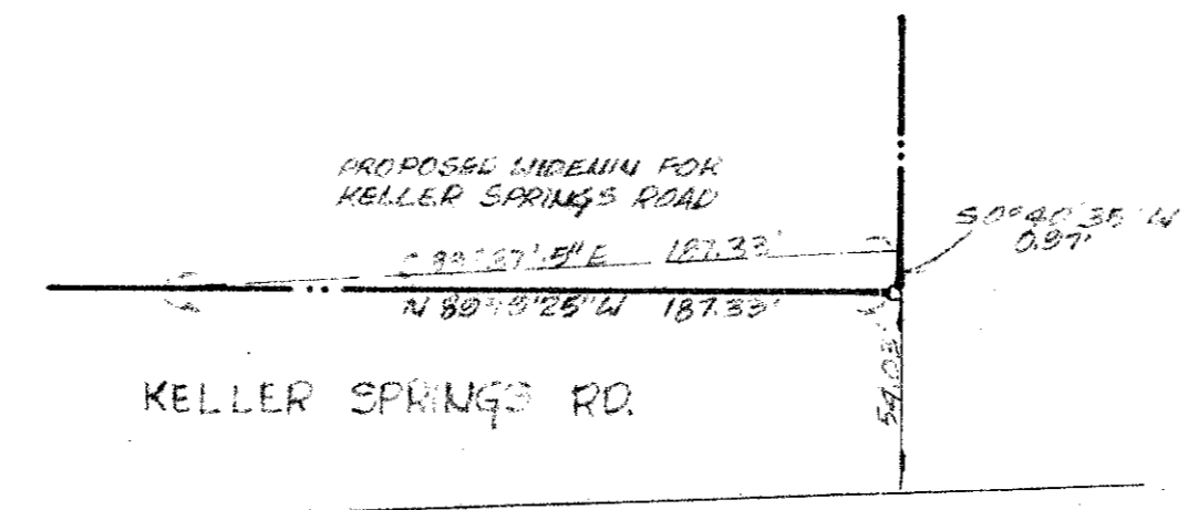
DETAIL (No. 2-16)
