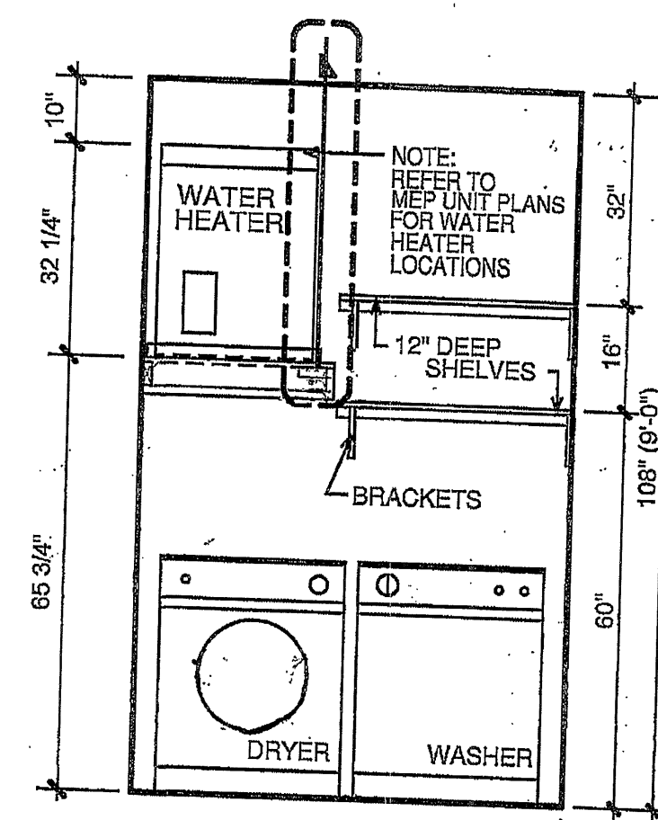
SUSPENDED WATER HEATER SHELF
