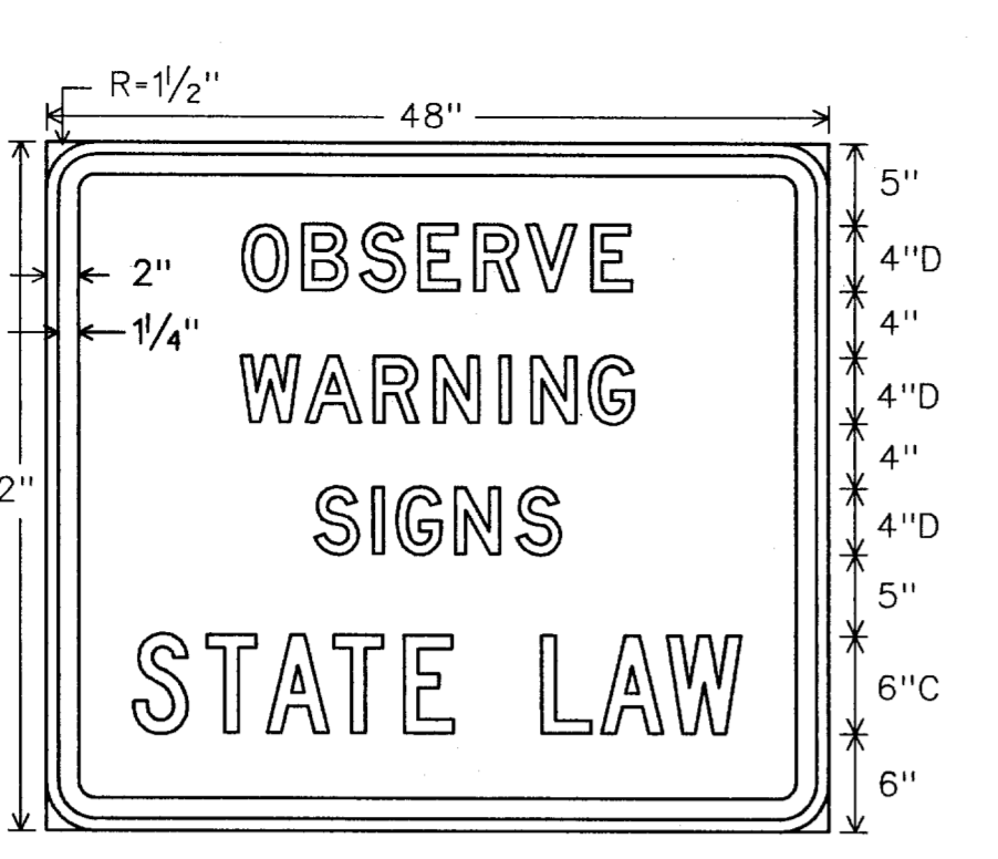
R20-3 48" X 42" Letters - Black Border - Black Background - White Refl.
