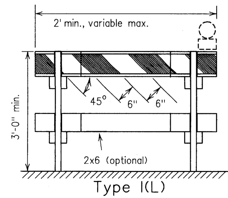
For Type I and II Barricades, both sides of the rails shall have reflective orange and reflective white striping.
