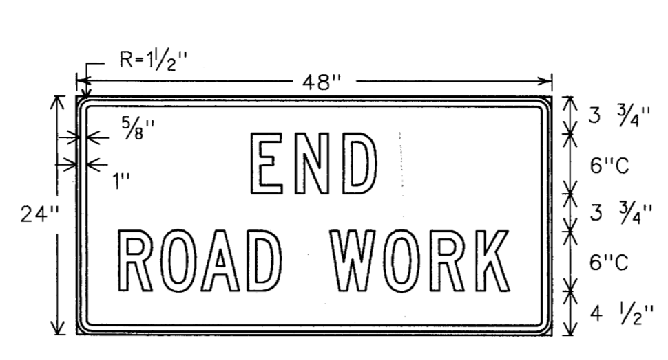
G20-2a 48" X 24" Letters - Black Border - Black Background - Orange Refl.
