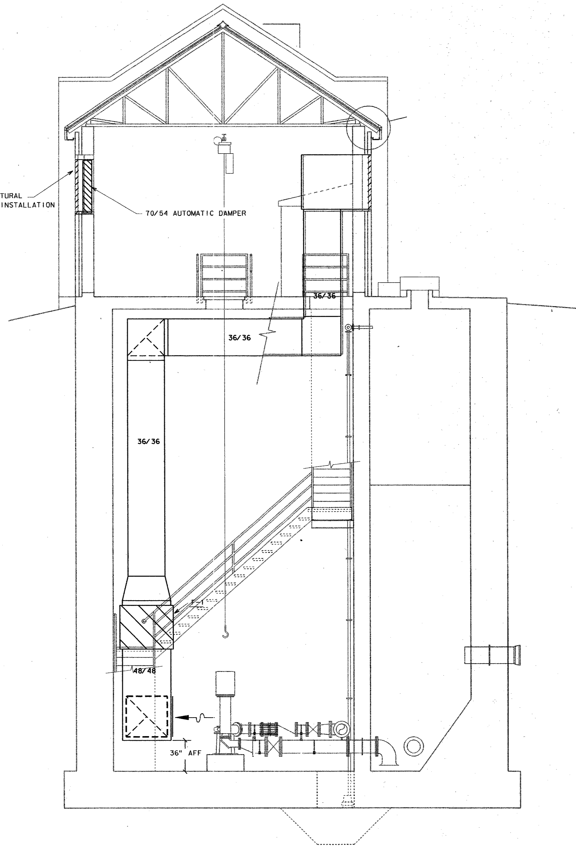
SECTION B 1/4" = 1'-0" (53)
