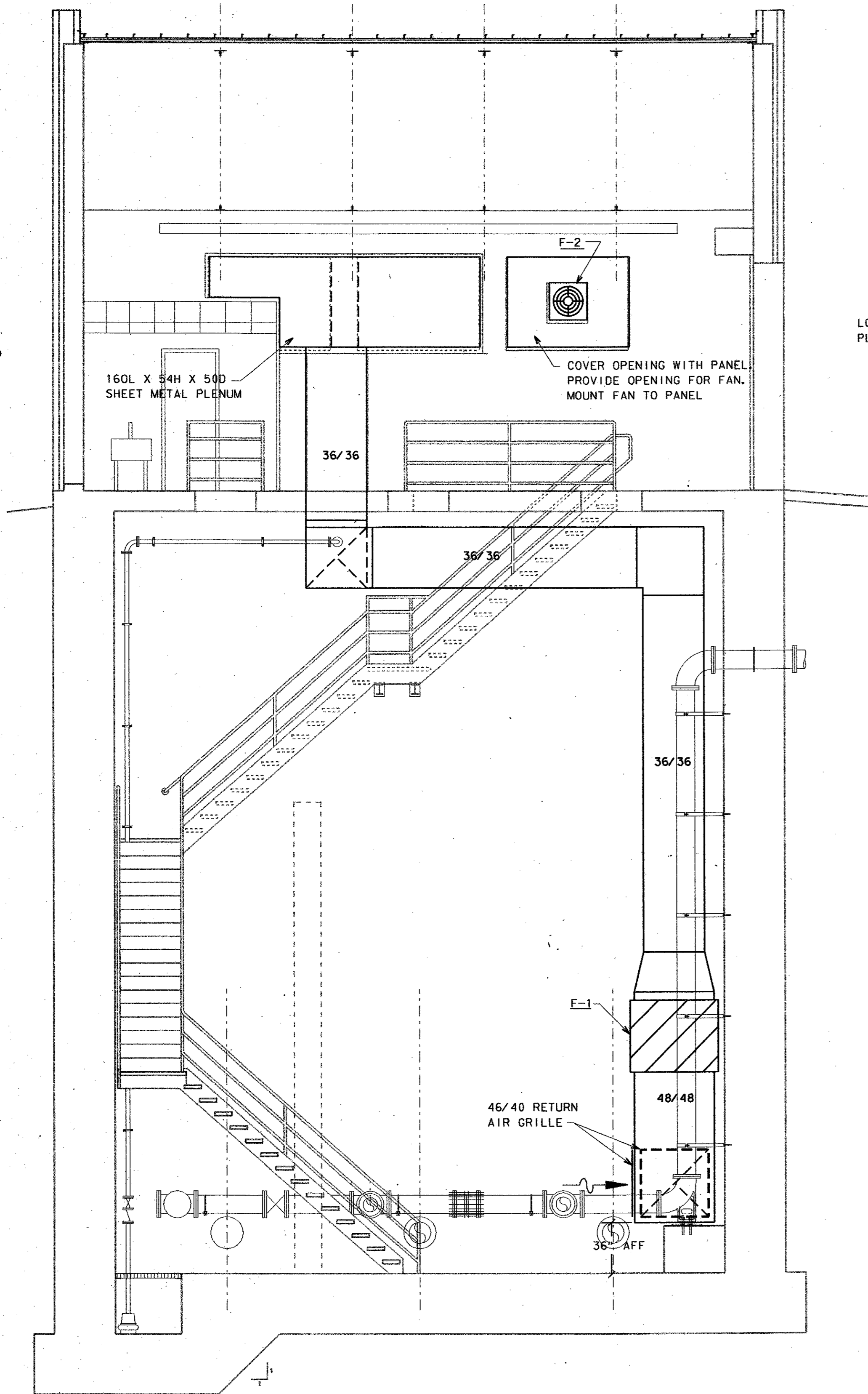
SECTION A 1/4" = 1'-0" (53)
