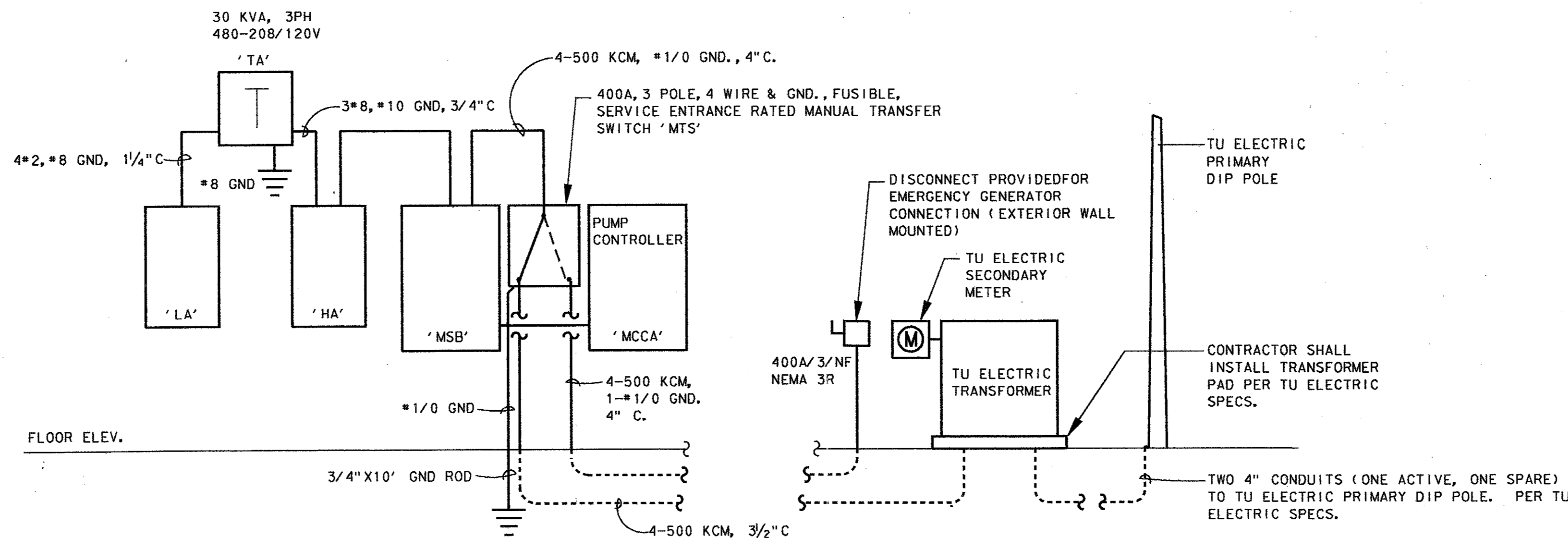
C ELECTRICAL RISER DIAGRAM SCALE: NO SCALE
