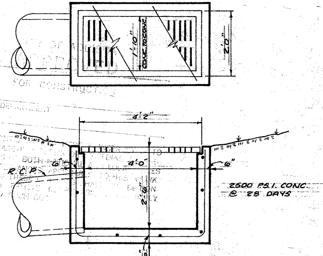
GRATE INLET DETAIL
