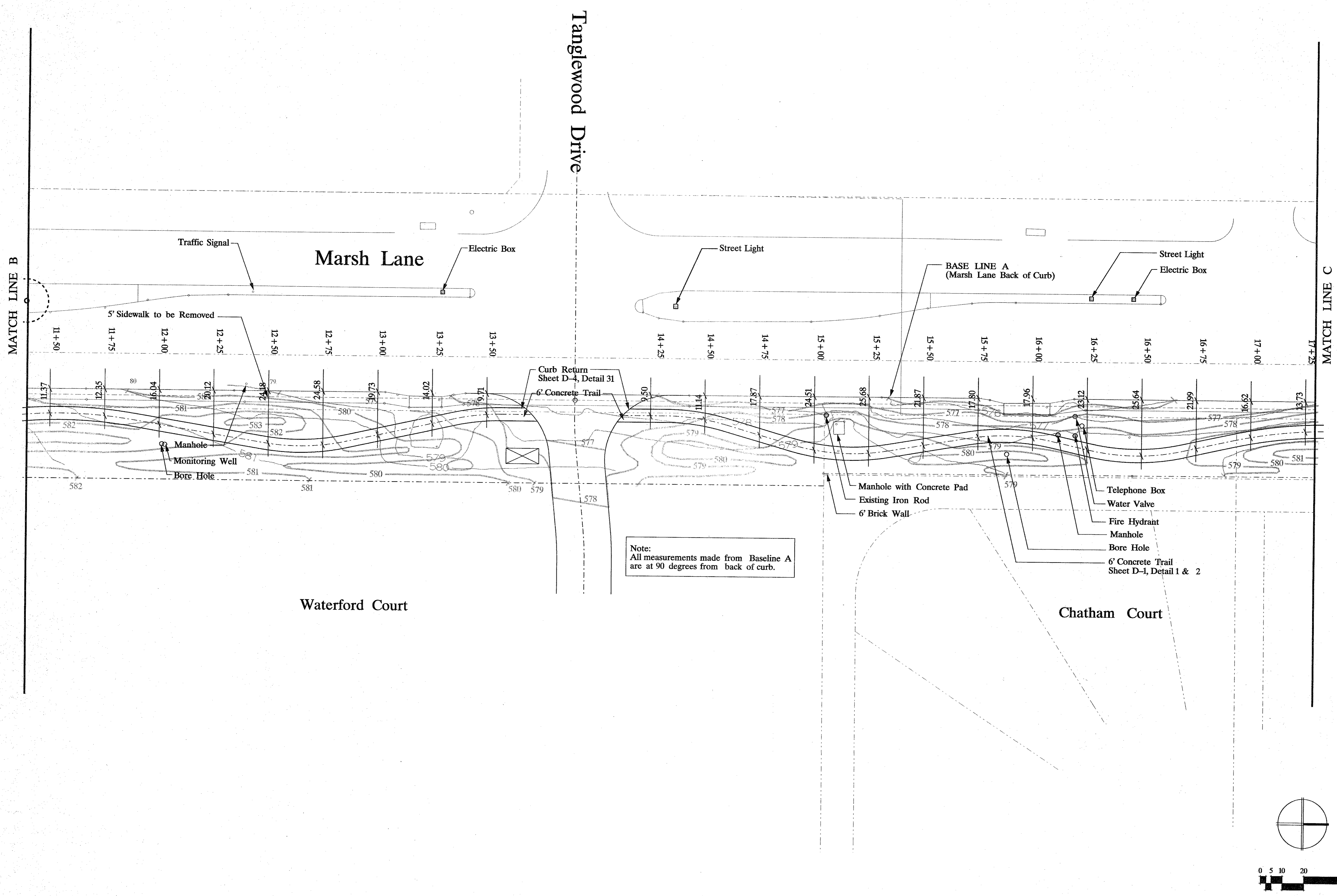
Layout and Dimensioning Plan Area Three
