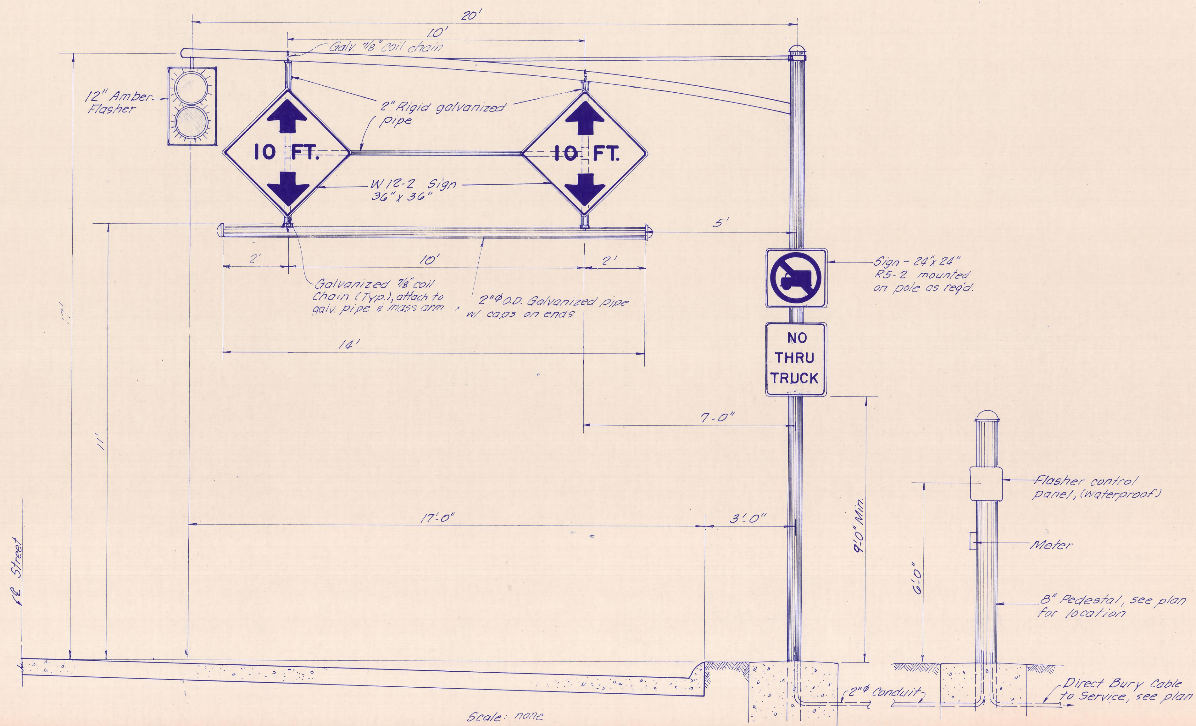
LOCATION PLAN Scale: 1"=20'
