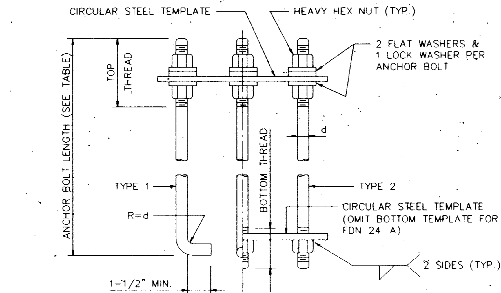
HOOKED ANCHOR (TYPE 1) NUT ANCHOR (TYPE 2) ANCHOR BOLT ASSEMBLY
