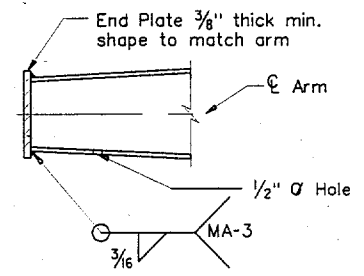
PLATE WELD DETAIL
