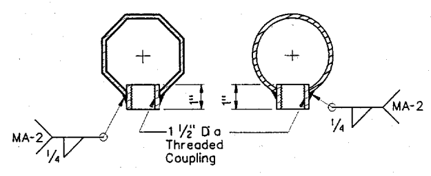
COUPLING DETAILS
