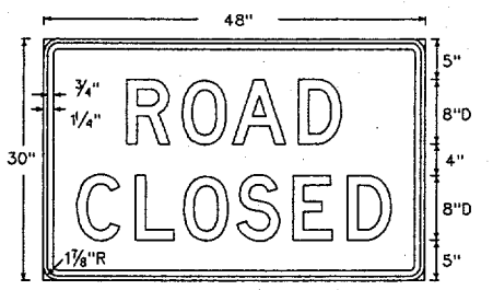
R11-2 Letters - Black Border - Black 48" X 30" Background - White Refl.
