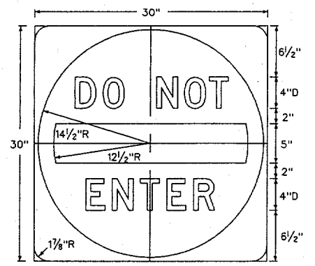
R5-1 Letters - White Refl. Bar - White Refl. Border - White Refl. 30" X 30" Background - Red Refl.
