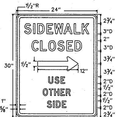
R5-8T Letters - Black Symbol - Black Border - Black 24" X 30" Background - White Refl.
