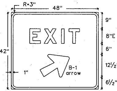
E5-1a Letters - White Refl. Numerals - White Refl. Symbol - White Refl. 48" X 42" Background - Green Refl.
