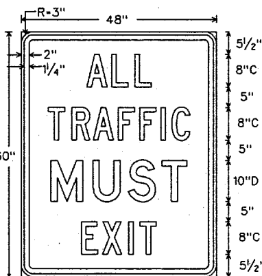
R3-22 Letters - Black Border - Black 48" X 60" Background - White Refl.
