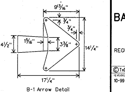
B-1 Arrow Detail
