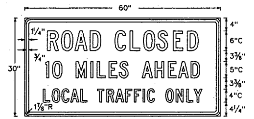
R11-3a Letters - Black Numerals - Black Border - Black 60" X 30" Background - White Refl.
