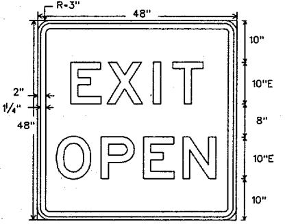
E5-2 Letters - Black Border - Black 48" X 48" Background - Orange Refl.
