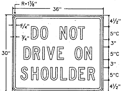
R4-3a Letters - Black Border - Black 36" X 30" Background - White Refl.
