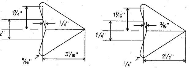
R20-5 Letters - Black Border - Black 24" X 12" Background - White Refl.
