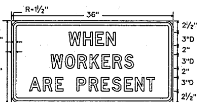
ER20-5 Letters - Black Border - Black 36" X 18" Background - White Refl.
