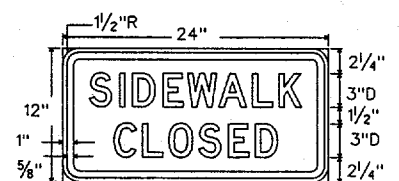
R5-8 Letters - Black Border - Black 24" X 12" Background - White Refl.
