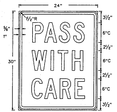
R4-2 Letters - Black Border - Black 24" X 30" Background - White Refl.
