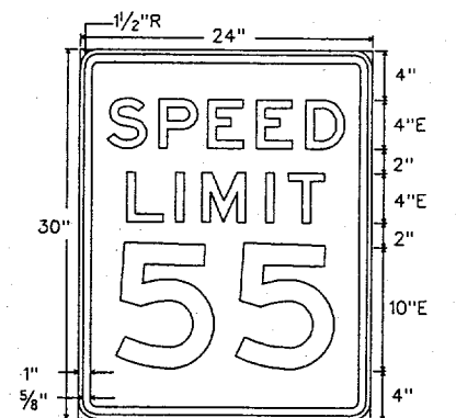
R2-1 Letters - Black Border - Black 24" X 30" Background - White Refl.
