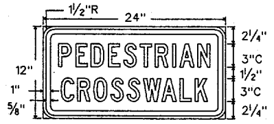
R5-7 Letters - Black Border - Black 24" X 12" Background - White Refl.
