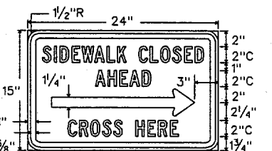
R5-9a Letters - Black Symbol - Black Border - Black 24" X 15" Background - White Refl.
