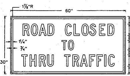
R11-4 Letters - Black Border - Black 60" X 30" Background - White Refl.
