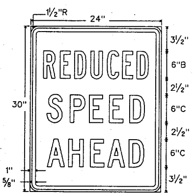
R2-5a Letters - Black Border - Black 24" X 30" Background - White Refl.
