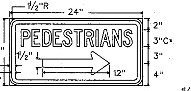
R5-7T Letters - Black Symbol - Black Border - Black 24" X 12" Background - White Refl.
