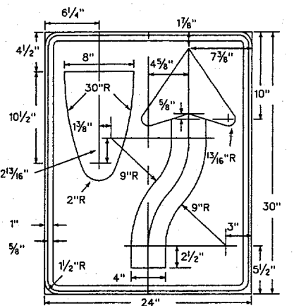
R4-7 Symbol - Black (R4-8) Border - Black 24" X 30" Background - White Refl.
