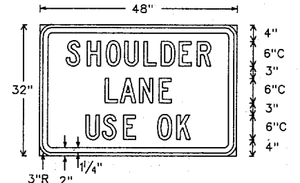
R4-3d Letters - Black Border - Black 48" X 32" Background - White Refl.
