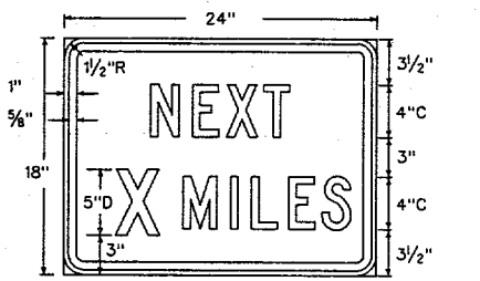
R20-1 Letters - Black Border - Black 24" X 18" Background - White Refl.
