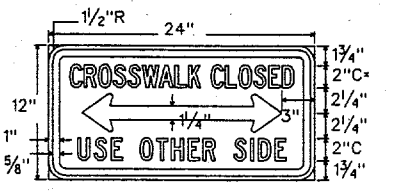
R5-9 Letters - Black Symbol - Black Border - Black 24" X 12" Background - White Refl.
