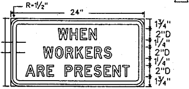
R20-5 Letters - Black Border - Black 24" X 12" Background - White Refl.
