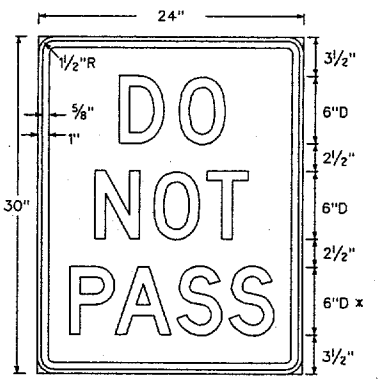
R4-1 Letters - Black Border - Black 24" X 30" Background - White Refl. x reduce spacing 40%
