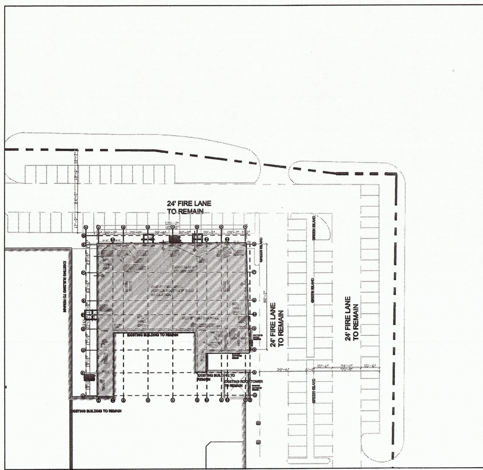
S: 1"=50'-0"
