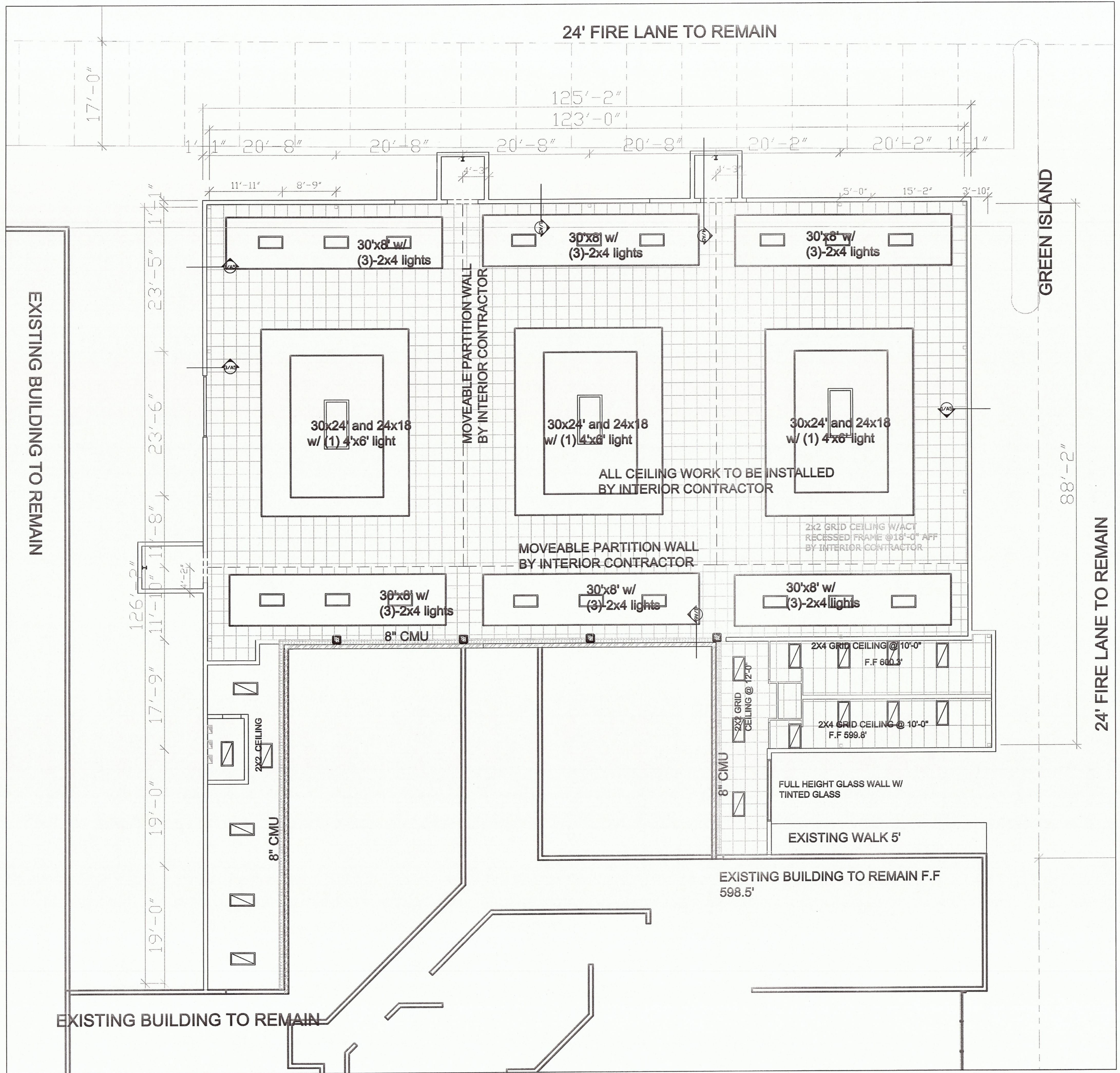
CEILING PLAN S: 1/8"=1'-0"
