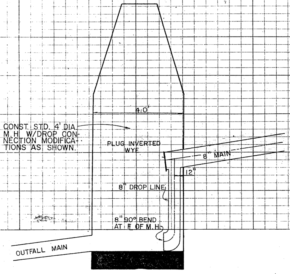
DROP MANHOLE DETAIL NO SCALE
