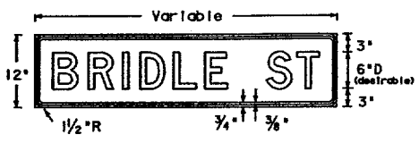
M4-9N Variable X 12" Letters - Black Border - Black Background - Orange Refl.
