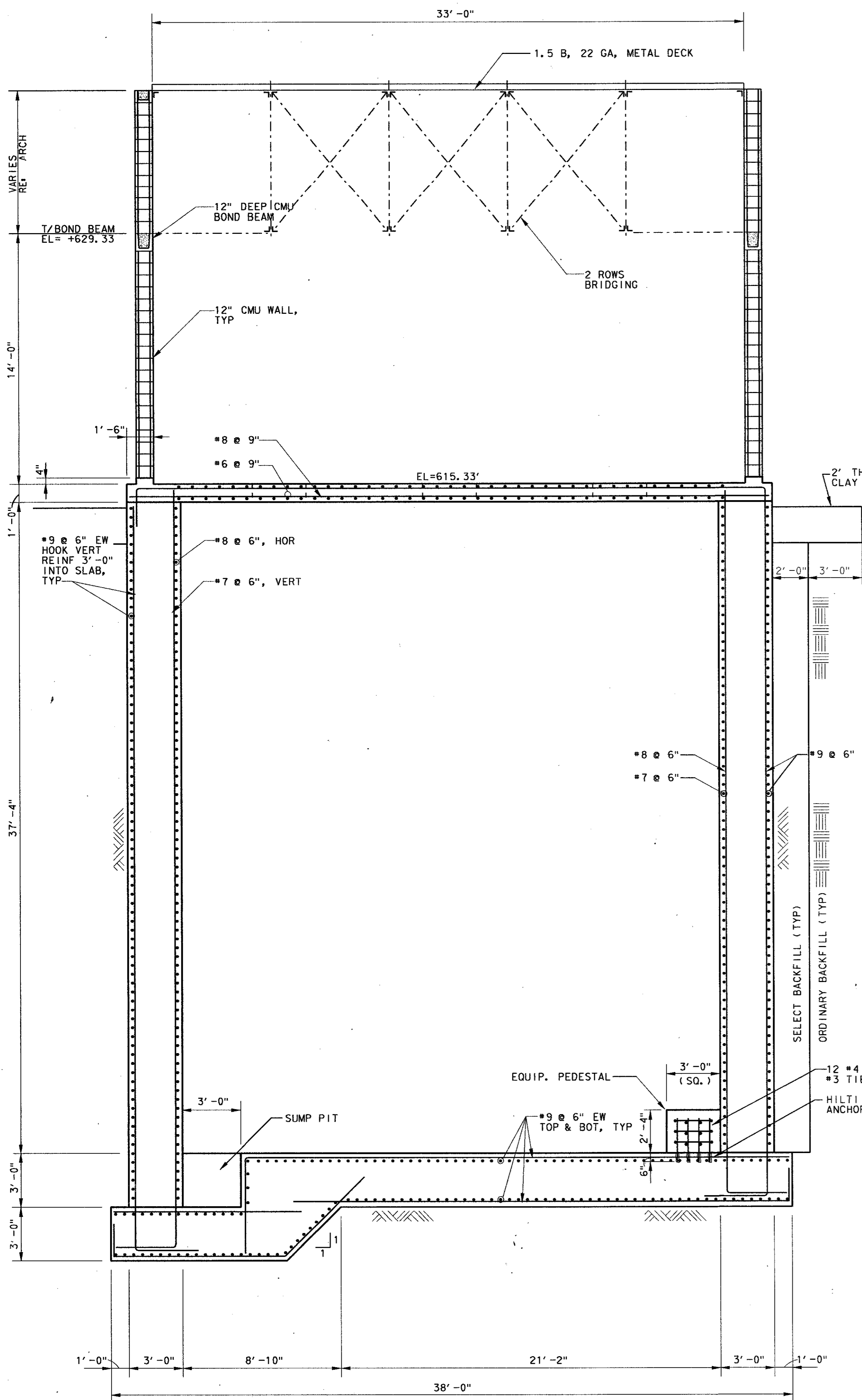
SECTION A 1/4" = 1' - 0"
